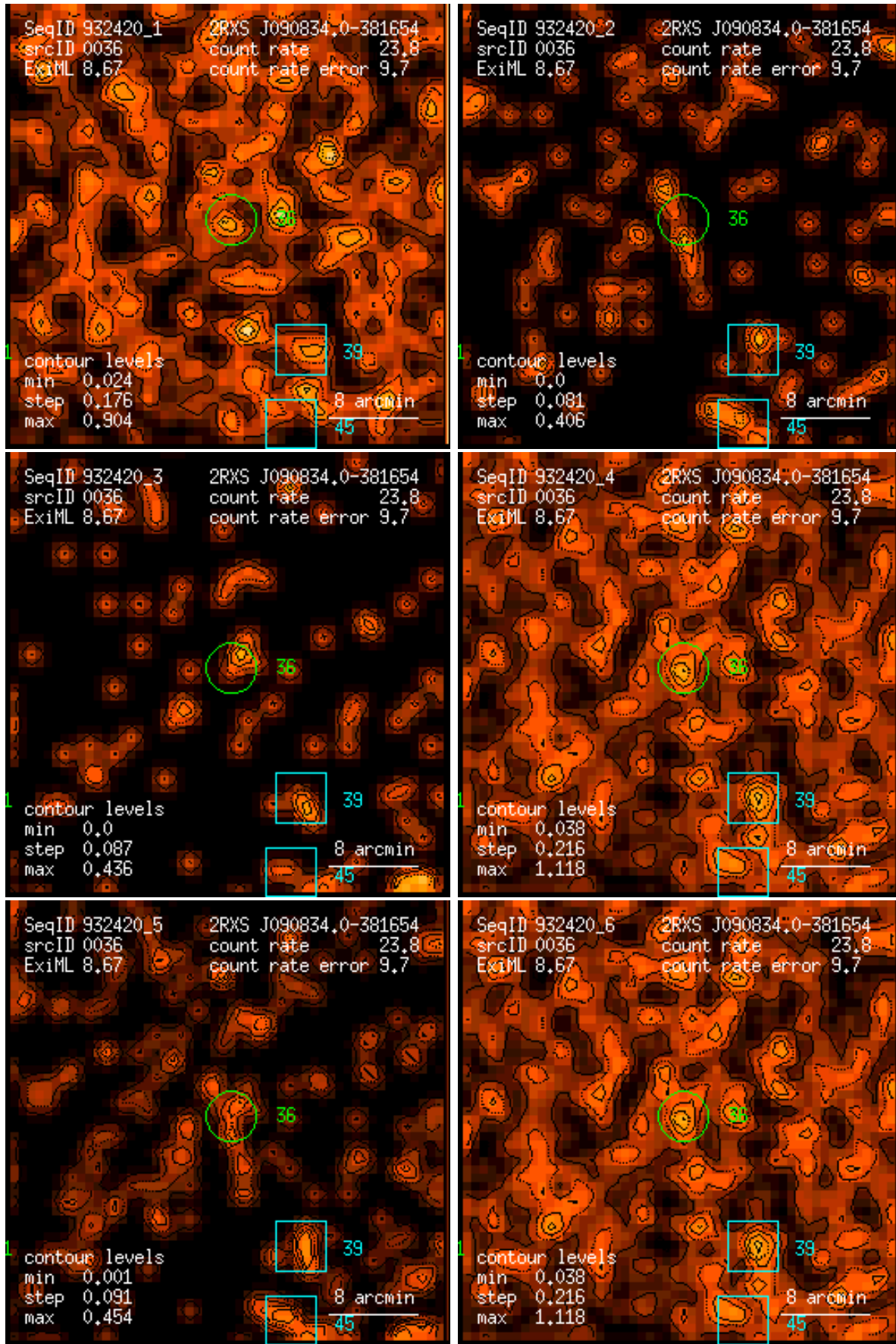
Figure 36: RASS 932420: detection 0036: band rate images, Gaussian filter: (1) PSPC channels 11 – 41, (2) 52 – 90, (3) 91 – 201, (4) 11 – 235, (5) 52 – 201, (6) 11 – 201. Broad band rates in counts/ks. Band rate contour levels in counts/ks/arcmin 2 .
