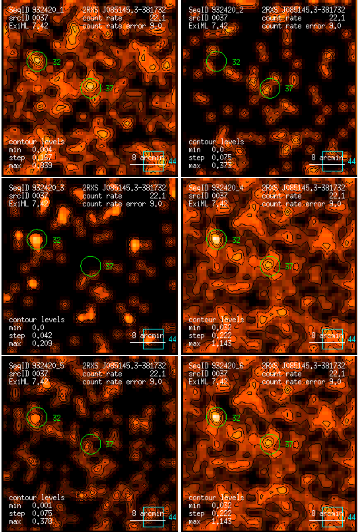
Figure 37: RASS 932420: detection 0037: band rate images, Gaussian filter: (1) PSPC channels 11 – 41, (2) 52 – 90, (3) 91 – 201, (4) 11 – 235, (5) 52 – 201, (6) 11 – 201. Broad band rates in counts/ks. Band rate contour levels in counts/ks/arcmin 2 .
