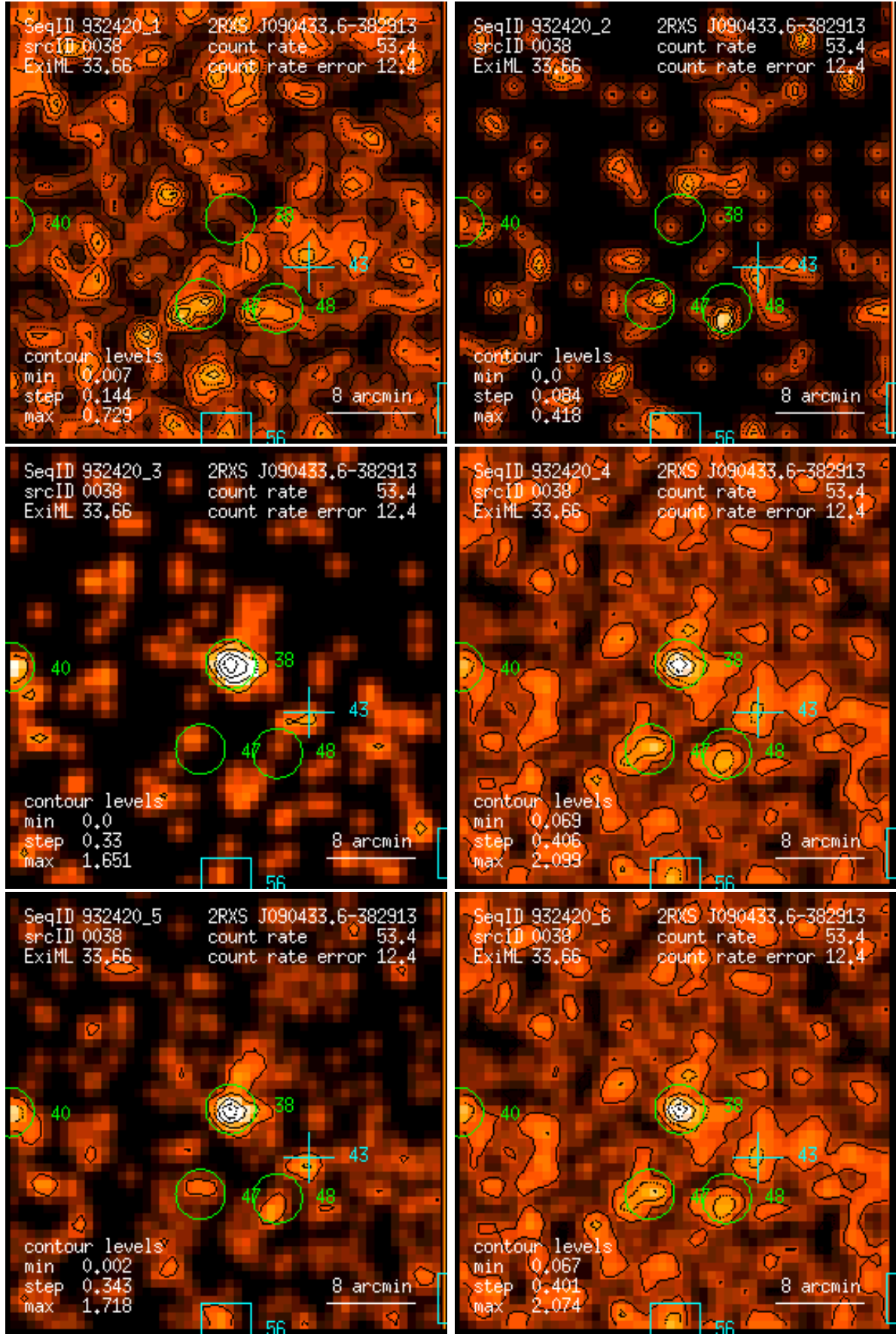
Figure 38: RASS 932420: detection 0038: band rate images, Gaussian filter: (1) PSPC channels 11 – 41, (2) 52 – 90, (3) 91 – 201, (4) 11 – 235, (5) 52 – 201, (6) 11 – 201. Broad band rates in counts/ks. Band rate contour levels in counts/ks/arcmin 2 .
