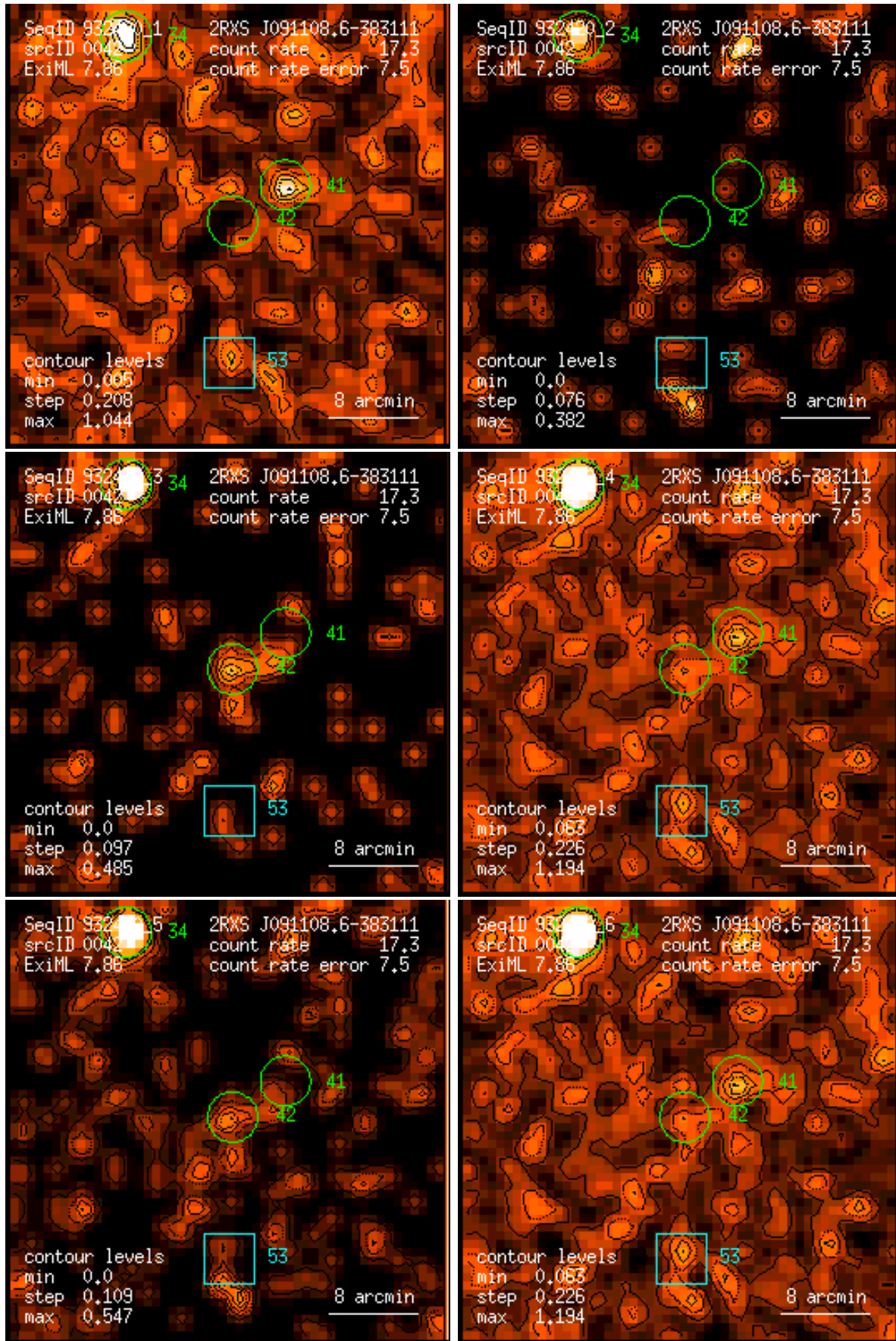
Figure 42: RASS 932420: detection 0042: band rate images, Gaussian filter: (1) PSPC channels 11 – 41, (2) 52 – 90, (3) 91 – 201, (4) 11 – 235, (5) 52 – 201, (6) 11 – 201. Broad band rates in counts/ks. Band rate contour levels in counts/ks/arcmin 2 .
