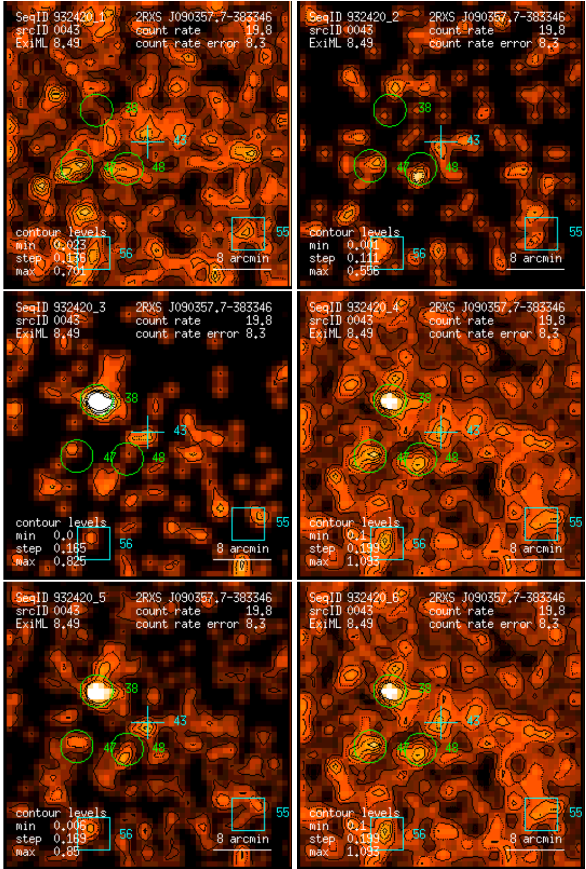
Figure 43: RASS 932420: detection 0043: band rate images, Gaussian filter: (1) PSPC channels 11 – 41, (2) 52 – 90, (3) 91 – 201, (4) 11 – 235, (5) 52 – 201, (6) 11 – 201. Broad band rates in counts/ks. Band rate contour levels in counts/ks/arcmin 2 .
