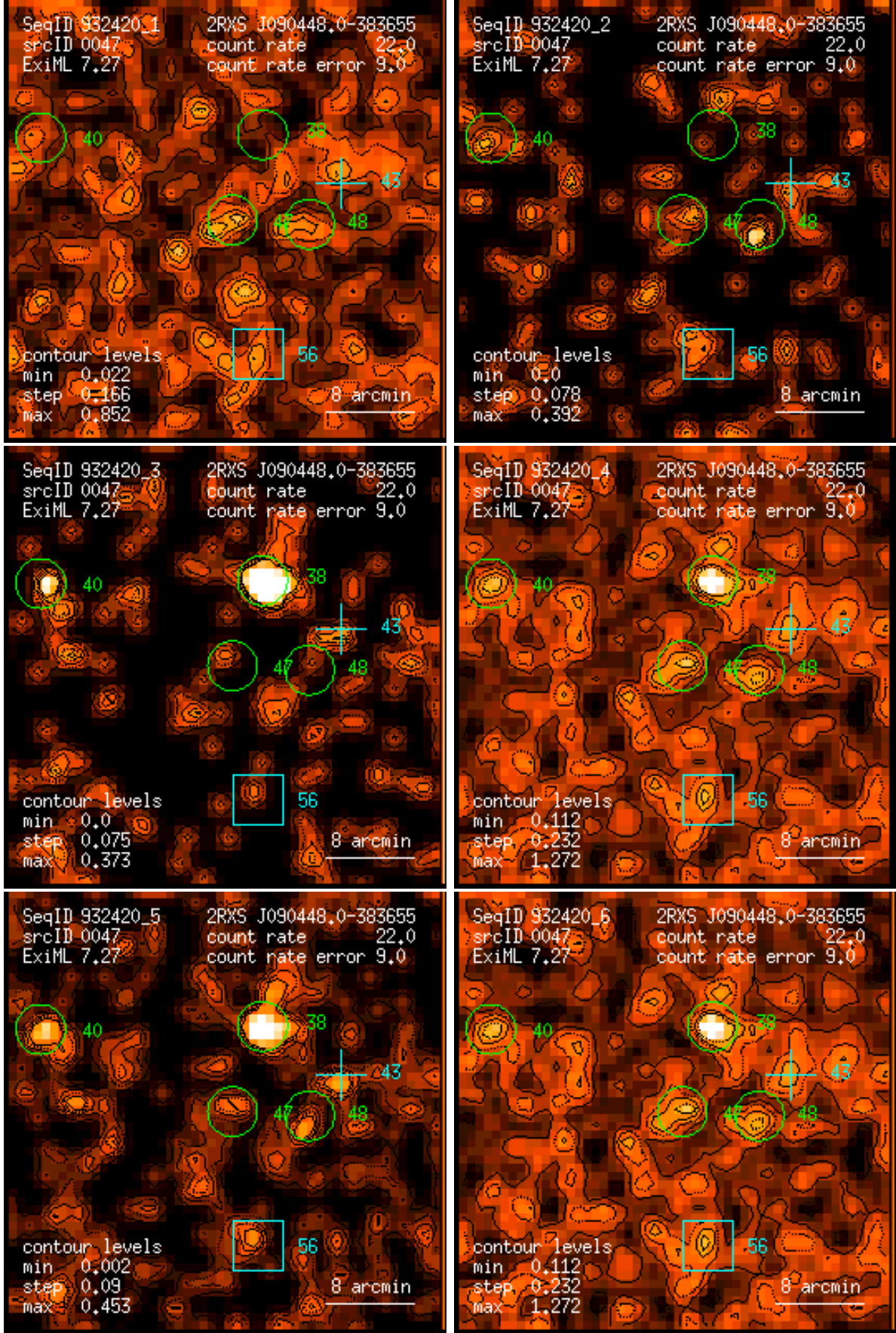
Figure 47: RASS 932420: detection 0047: band rate images, Gaussian filter: (1) PSPC channels 11 – 41, (2) 52 – 90, (3) 91 – 201, (4) 11 – 235, (5) 52 – 201, (6) 11 – 201. Broad band rates in counts/ks. Band rate contour levels in counts/ks/arcmin 2 .
