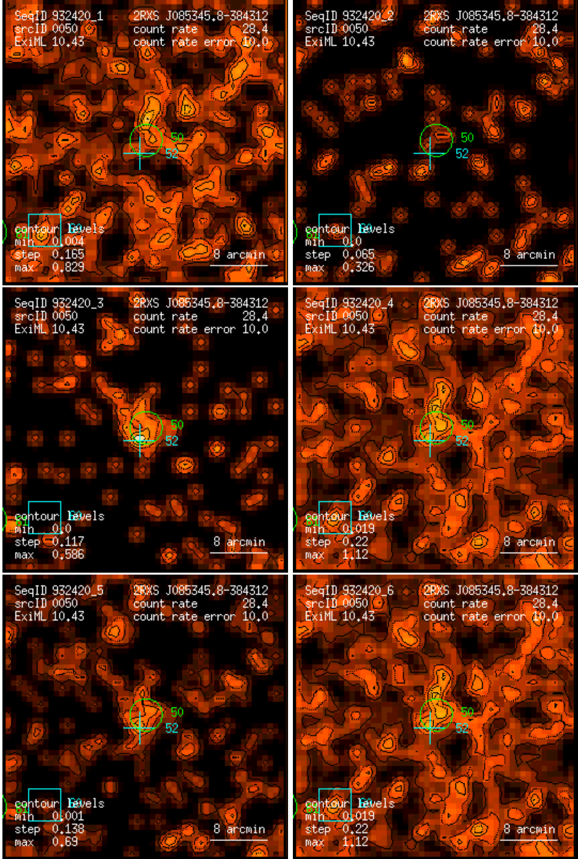
Figure 50: RASS 932420: detection 0050: band rate images, Gaussian filter: (1) PSPC channels 11 – 41, (2) 52 – 90, (3) 91 – 201, (4) 11 – 235, (5) 52 – 201, (6) 11 – 201. Broad band rates in counts/ks. Band rate contour levels in counts/ks/arcmin 2 .
