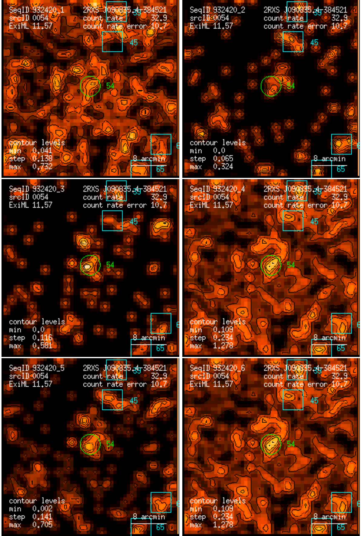
Figure 54: RASS 932420: detection 0054: band rate images, Gaussian filter: (1) PSPC channels 11 – 41, (2) 52 – 90, (3) 91 – 201, (4) 11 – 235, (5) 52 – 201, (6) 11 – 201. Broad band rates in counts/ks. Band rate contour levels in counts/ks/arcmin 2 .
