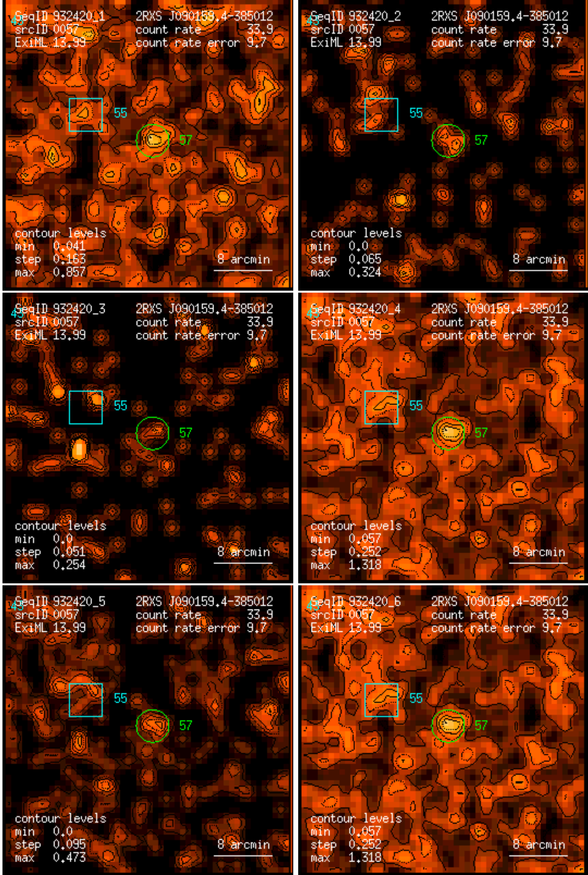
Figure 57: RASS 932420: detection 0057: band rate images, Gaussian filter: (1) PSPC channels 11 – 41, (2) 52 – 90, (3) 91 – 201, (4) 11 – 235, (5) 52 – 201, (6) 11 – 201. Broad band rates in counts/ks. Band rate contour levels in counts/ks/arcmin 2 .
