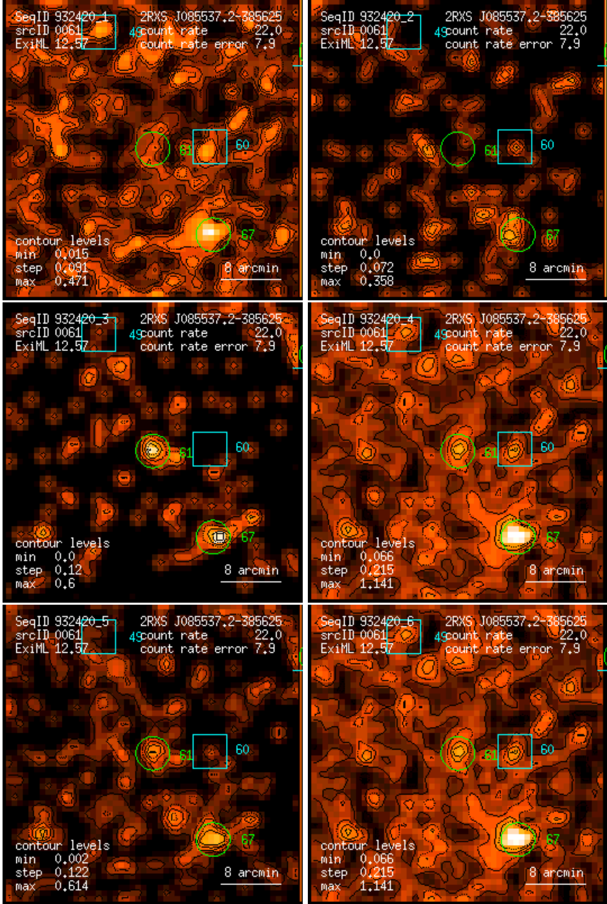
Figure 61: RASS 932420: detection 0061: band rate images, Gaussian filter: (1) PSPC channels 11 – 41, (2) 52 – 90, (3) 91 – 201, (4) 11 – 235, (5) 52 – 201, (6) 11 – 201. Broad band rates in counts/ks. Band rate contour levels in counts/ks/arcmin 2 .
