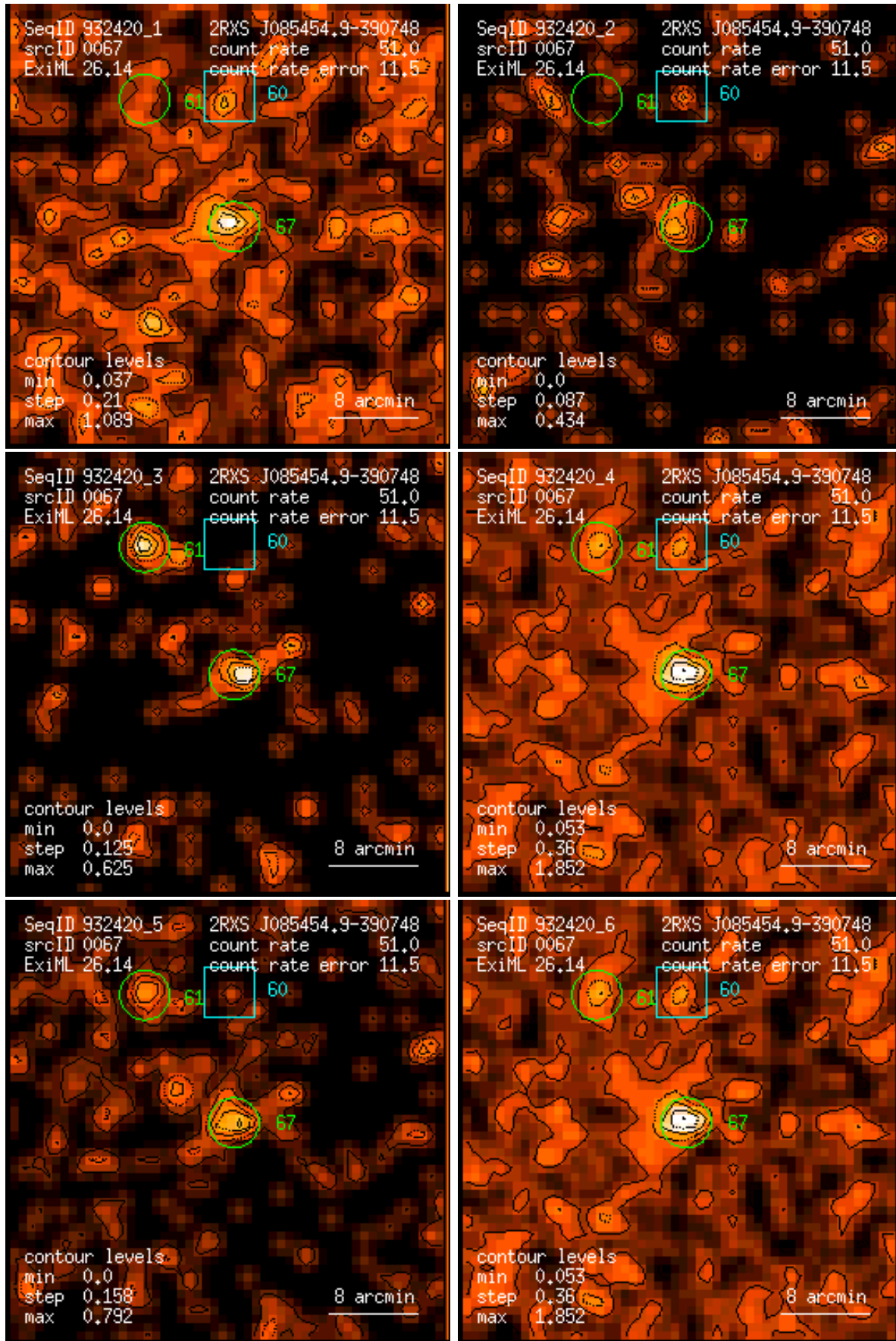
Figure 67: RASS 932420: detection 0067: band rate images, Gaussian filter: (1) PSPC channels 11 – 41, (2) 52 – 90, (3) 91 – 201, (4) 11 – 235, (5) 52 – 201, (6) 11 – 201. Broad band rates in counts/ks. Band rate contour levels in counts/ks/arcmin 2 .
