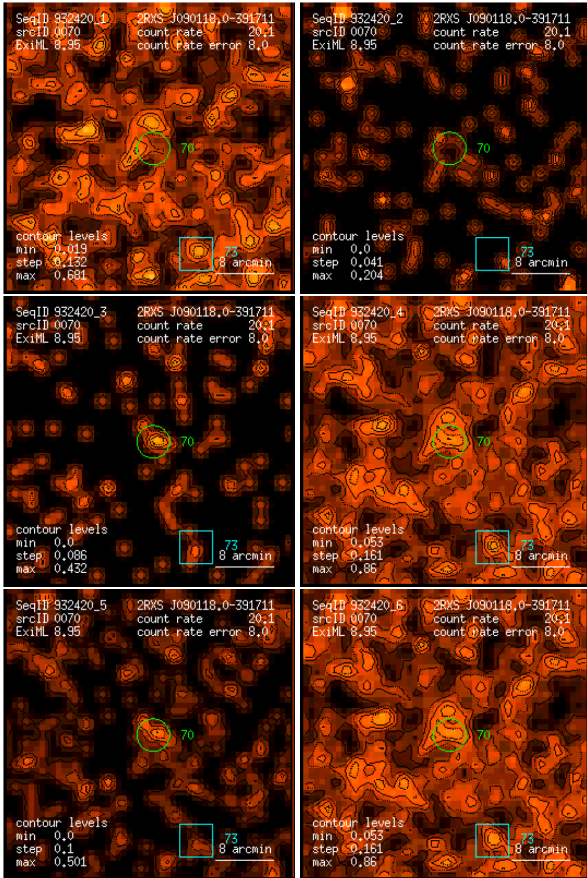
Figure 70: RASS 932420: detection 0070: band rate images, Gaussian filter: (1) PSPC channels 11 – 41, (2) 52 – 90, (3) 91 – 201, (4) 11 – 235, (5) 52 – 201, (6) 11 – 201. Broad band rates in counts/ks. Band rate contour levels in counts/ks/arcmin 2 .
