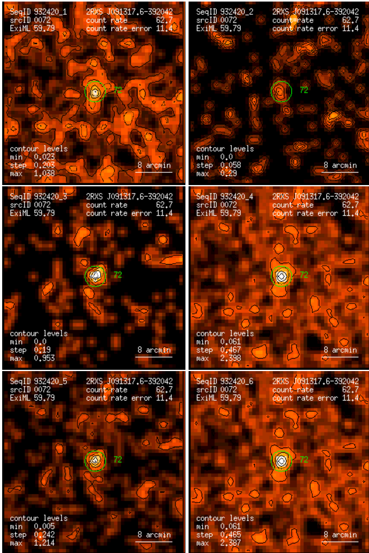
Figure 72: RASS 932420: detection 0072: band rate images, Gaussian filter: (1) PSPC channels 11 – 41, (2) 52 – 90, (3) 91 – 201, (4) 11 – 235, (5) 52 – 201, (6) 11 – 201. Broad band rates in counts/ks. Band rate contour levels in counts/ks/arcmin 2 .
