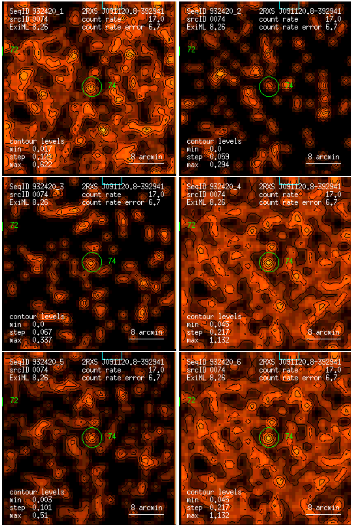
Figure 74: RASS 932420: detection 0074: band rate images, Gaussian filter: (1) PSPC channels 11 – 41, (2) 52 – 90, (3) 91 – 201, (4) 11 – 235, (5) 52 – 201, (6) 11 – 201. Broad band rates in counts/ks. Band rate contour levels in counts/ks/arcmin 2 .
