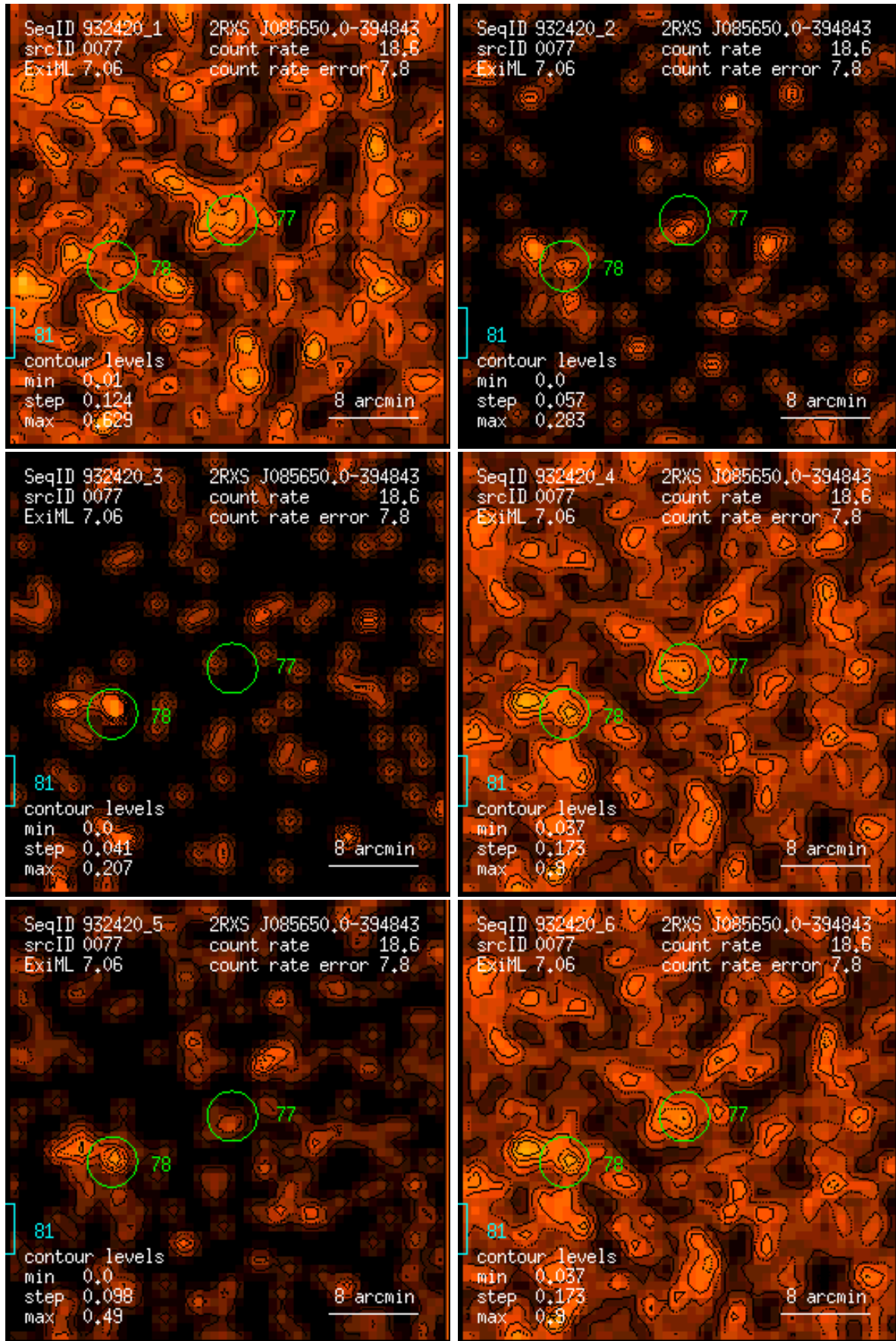
Figure 77: RASS 932420: detection 0077: band rate images, Gaussian filter: (1) PSPC channels 11 – 41, (2) 52 – 90, (3) 91 – 201, (4) 11 – 235, (5) 52 – 201, (6) 11 – 201. Broad band rates in counts/ks. Band rate contour levels in counts/ks/arcmin 2 .
