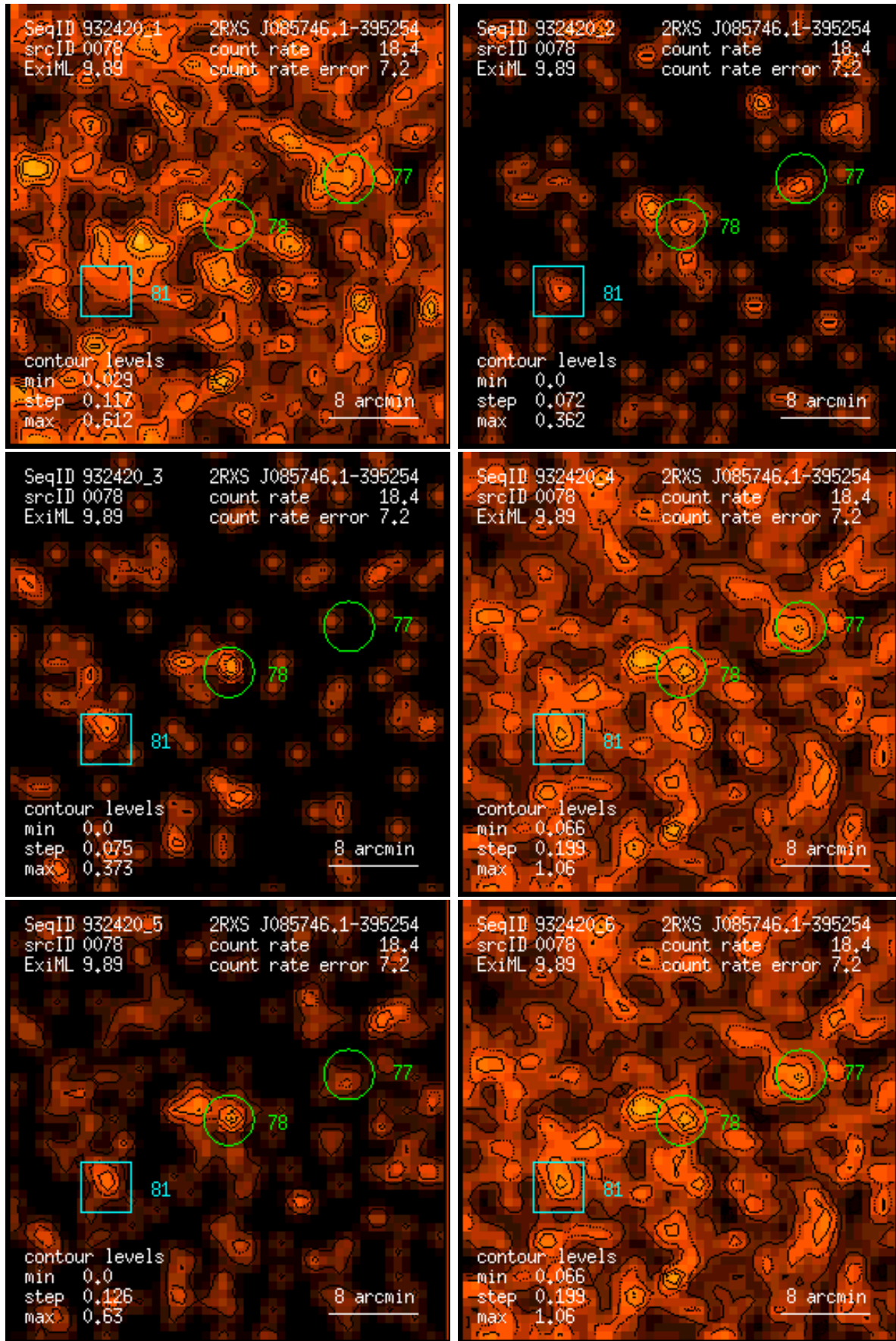
Figure 78: RASS 932420: detection 0078: band rate images, Gaussian filter: (1) PSPC channels 11 – 41, (2) 52 – 90, (3) 91 – 201, (4) 11 – 235, (5) 52 – 201, (6) 11 – 201. Broad band rates in counts/ks. Band rate contour levels in counts/ks/arcmin 2 .
