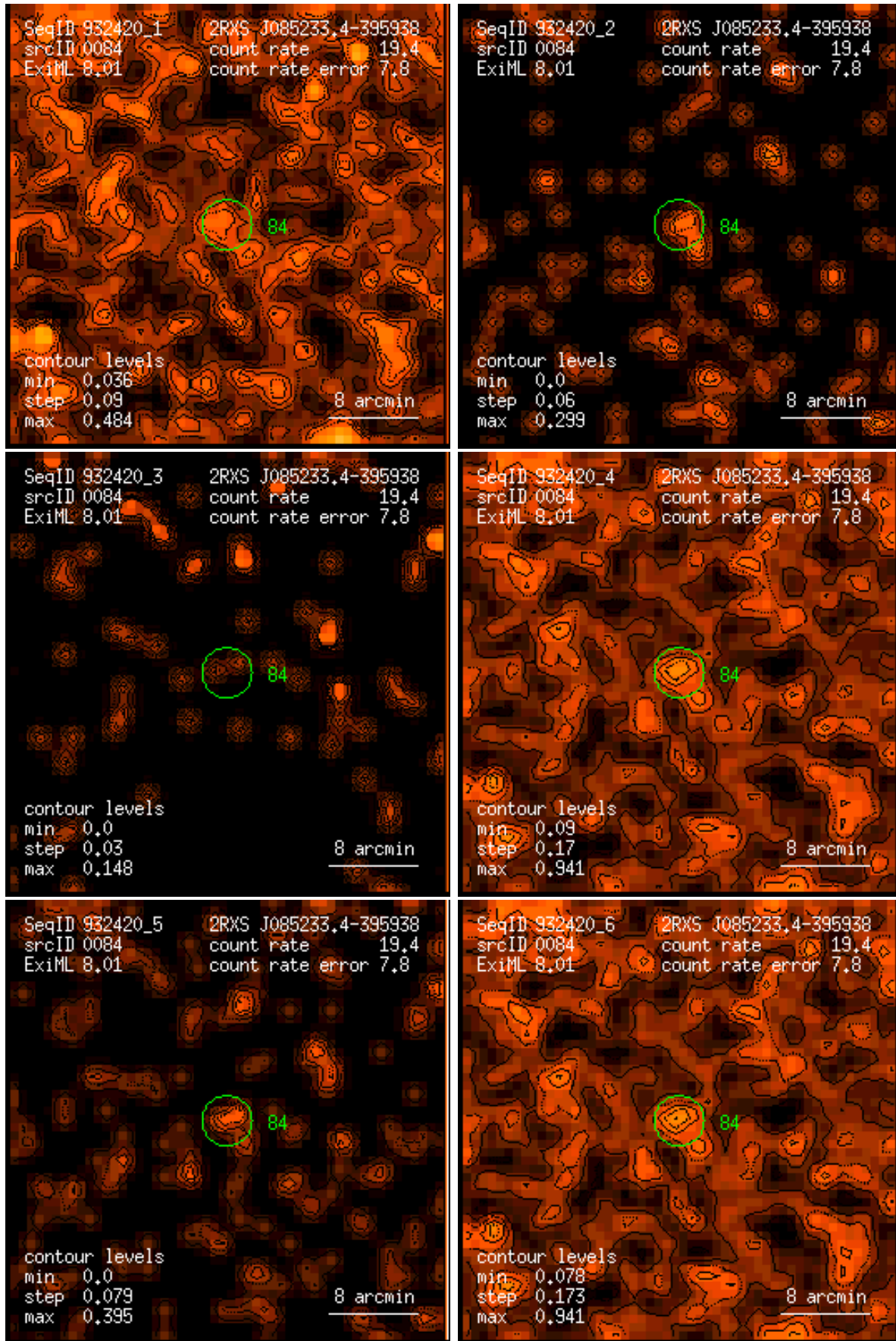
Figure 84: RASS 932420: detection 0084: band rate images, Gaussian filter: (1) PSPC channels 11 – 41, (2) 52 – 90, (3) 91 – 201, (4) 11 – 235, (5) 52 – 201, (6) 11 – 201. Broad band rates in counts/ks. Band rate contour levels in counts/ks/arcmin 2 .
