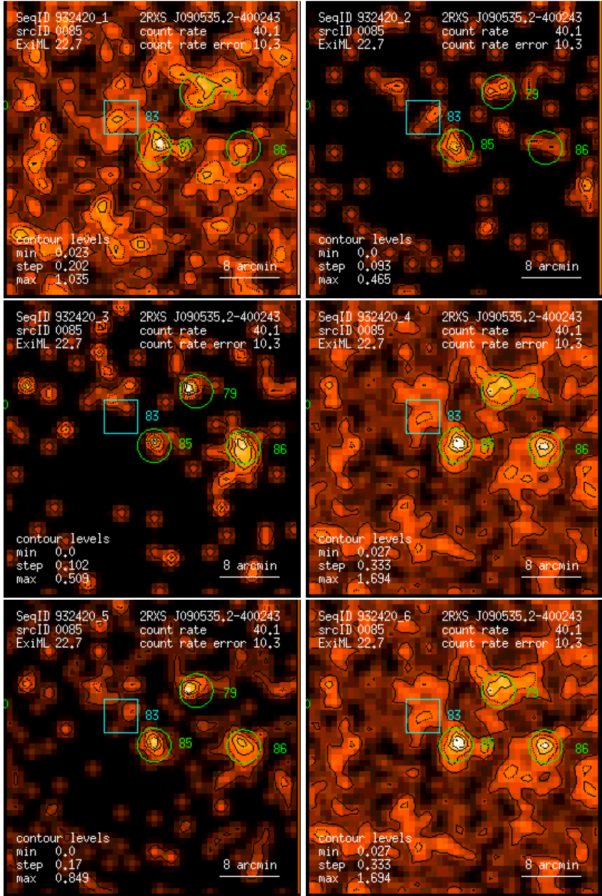
Figure 85: RASS 932420: detection 0085: band rate images, Gaussian filter: (1) PSPC channels 11 – 41, (2) 52 – 90, (3) 91 – 201, (4) 11 – 235, (5) 52 – 201, (6) 11 – 201. Broad band rates in counts/ks. Band rate contour levels in counts/ks/arcmin 2 .
