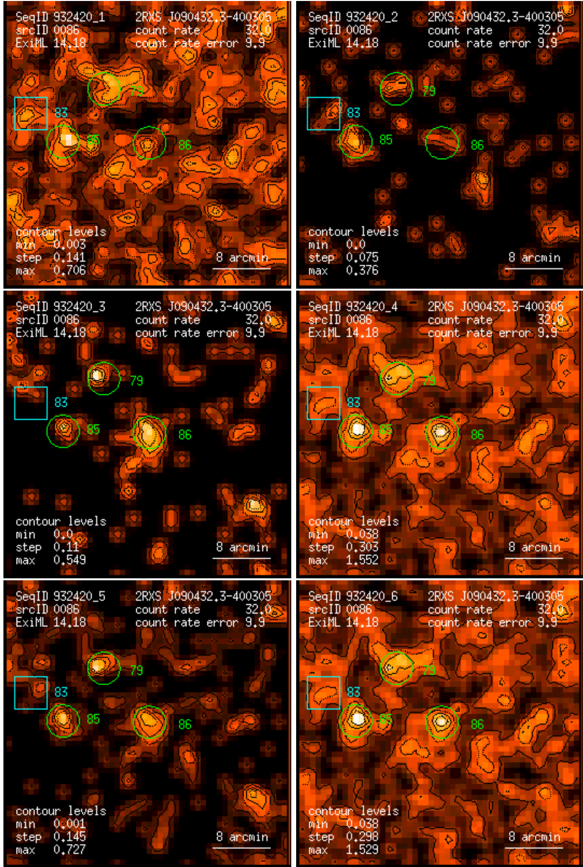
Figure 86: RASS 932420: detection 0086: band rate images, Gaussian filter: (1) PSPC channels 11 – 41, (2) 52 – 90, (3) 91 – 201, (4) 11 – 235, (5) 52 – 201, (6) 11 – 201. Broad band rates in counts/ks. Band rate contour levels in counts/ks/arcmin 2 .
