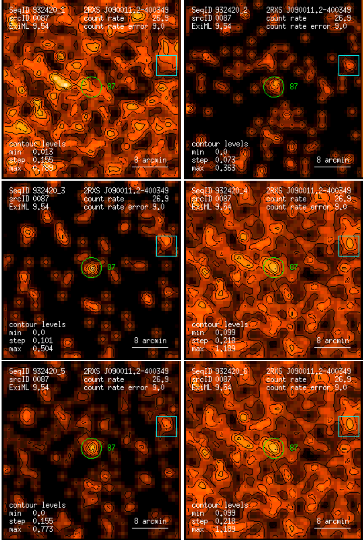
Figure 87: RASS 932420: detection 0087: band rate images, Gaussian filter: (1) PSPC channels 11 – 41, (2) 52 – 90, (3) 91 – 201, (4) 11 – 235, (5) 52 – 201, (6) 11 – 201. Broad band rates in counts/ks. Band rate contour levels in counts/ks/arcmin 2 .
