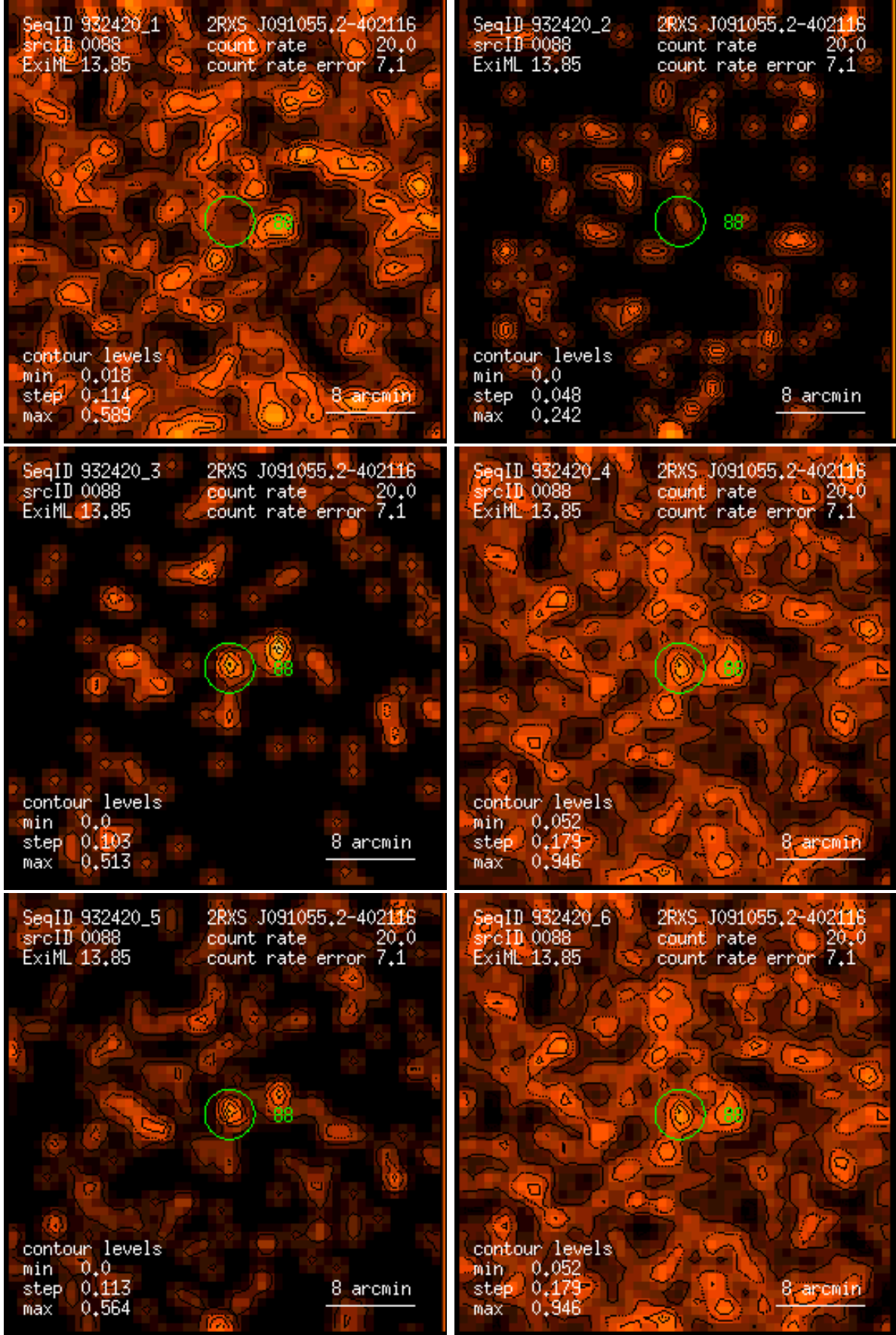
Figure 88: RASS 932420: detection 0088: band rate images, Gaussian filter: (1) PSPC channels 11 – 41, (2) 52 – 90, (3) 91 – 201, (4) 11 – 235, (5) 52 – 201, (6) 11 – 201. Broad band rates in counts/ks. Band rate contour levels in counts/ks/arcmin 2 .
