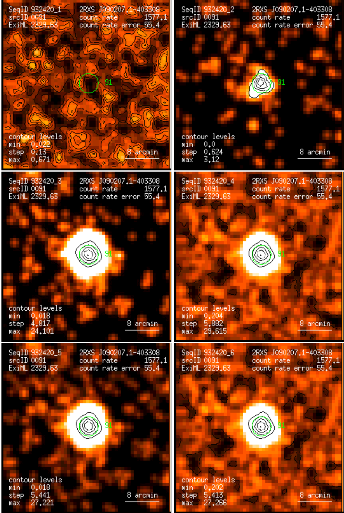
Figure 91: RASS 932420: detection 0091: band rate images, Gaussian filter: (1) PSPC channels 11 – 41, (2) 52 – 90, (3) 91 – 201, (4) 11 – 235, (5) 52 – 201, (6) 11 – 201. Broad band rates in counts/ks. Band rate contour levels in counts/ks/arcmin 2 .
