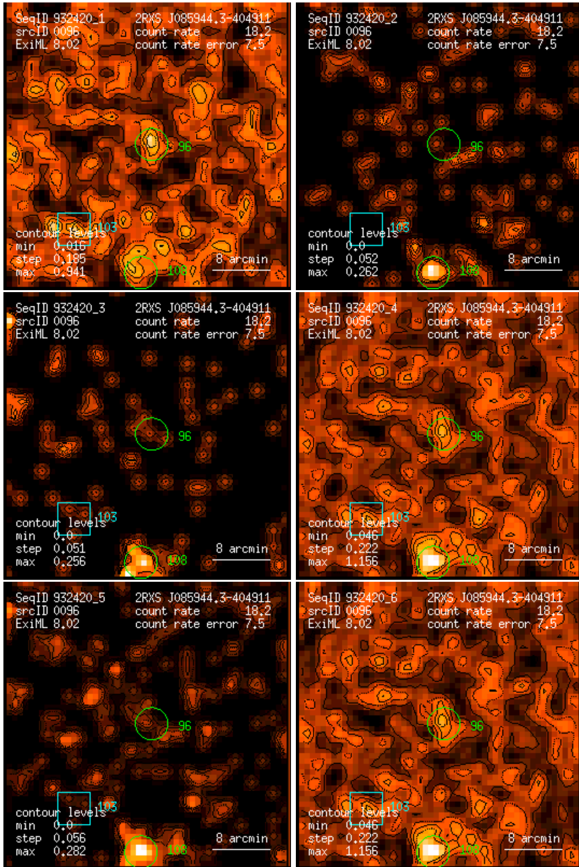
Figure 96: RASS 932420: detection 0096: band rate images, Gaussian filter: (1) PSPC channels 11 – 41, (2) 52 – 90, (3) 91 – 201, (4) 11 – 235, (5) 52 – 201, (6) 11 – 201. Broad band rates in counts/ks. Band rate contour levels in counts/ks/arcmin 2 .
