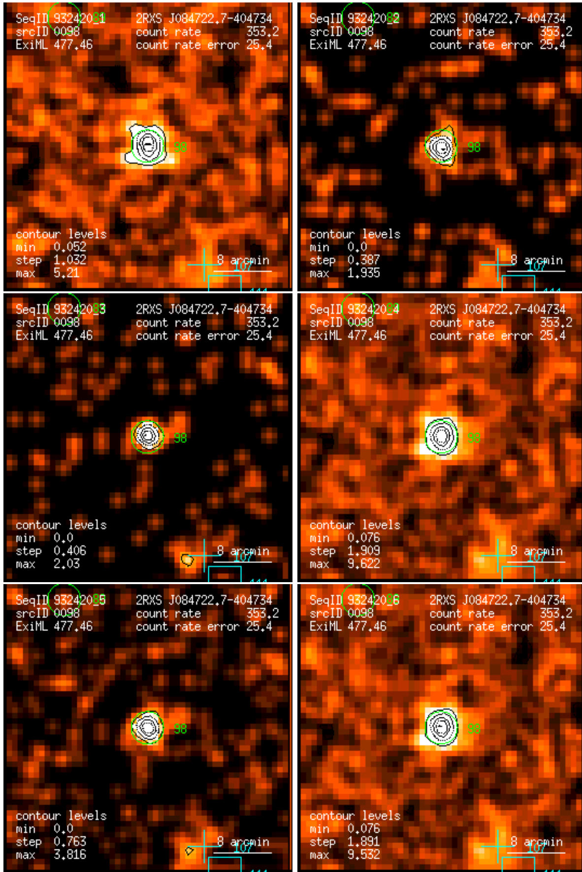
Figure 98: RASS 932420: detection 0098: band rate images, Gaussian filter: (1) PSPC channels 11 – 41, (2) 52 – 90, (3) 91 – 201, (4) 11 – 235, (5) 52 – 201, (6) 11 – 201. Broad band rates in counts/ks. Band rate contour levels in counts/ks/arcmin 2 .
