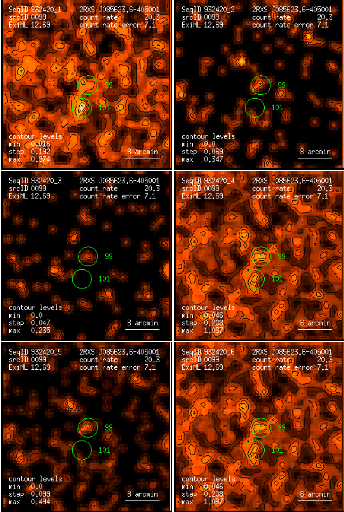
Figure 99: RASS 932420: detection 0099: band rate images, Gaussian filter: (1) PSPC channels 11 – 41, (2) 52 – 90, (3) 91 – 201, (4) 11 – 235, (5) 52 – 201, (6) 11 – 201. Broad band rates in counts/ks. Band rate contour levels in counts/ks/arcmin 2 .
