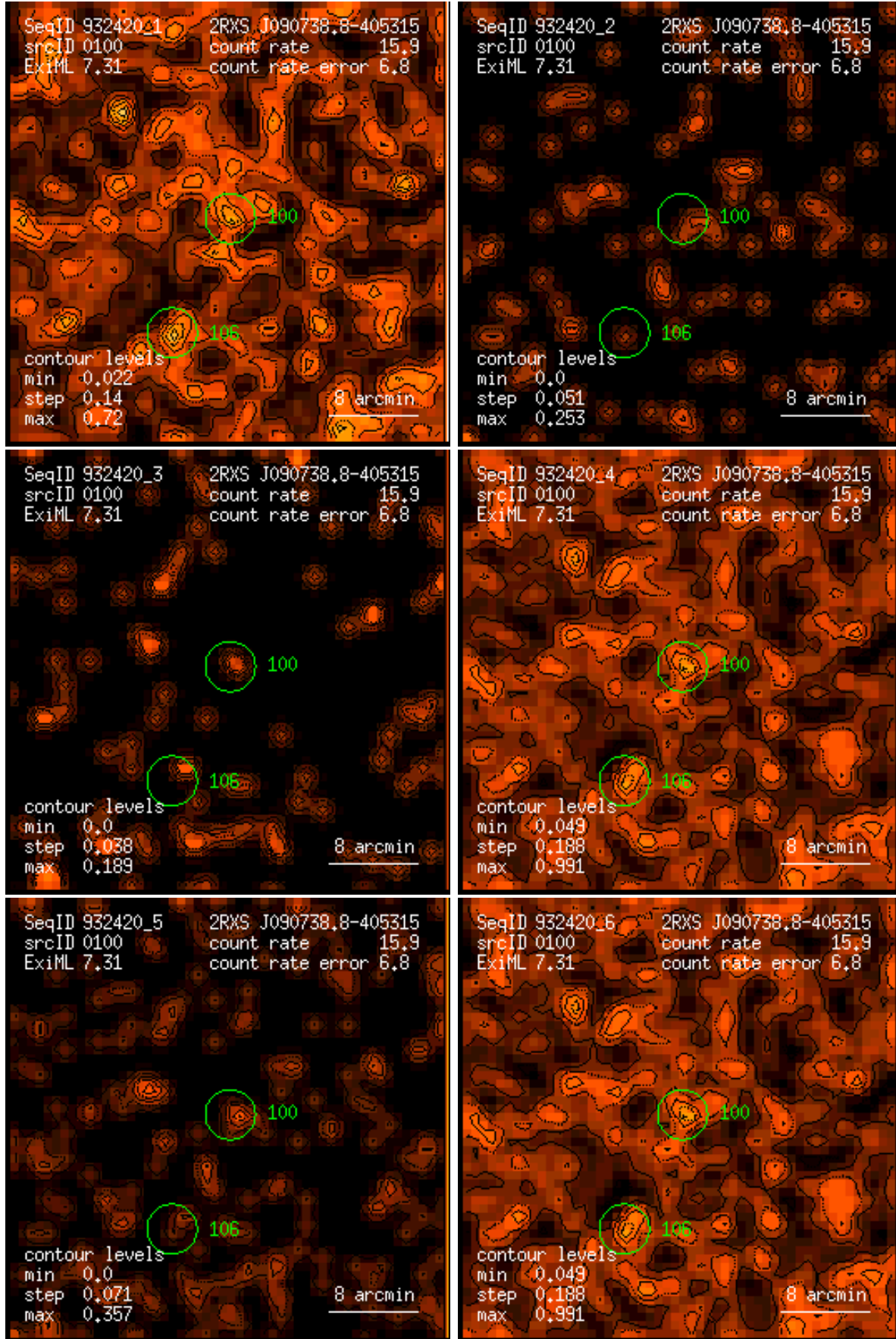
Figure 100: RASS 932420: detection 0100: band rate images, Gaussian filter: (1) PSPC channels 11 – 41, (2) 52 – 90, (3) 91 – 201, (4) 11 – 235, (5) 52 – 201, (6) 11 – 201. Broad band rates in counts/ks. Band rate contour levels in counts/ks/arcmin 2 .
