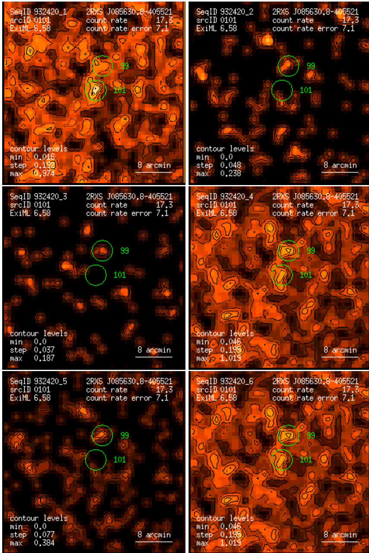
Figure 101: RASS 932420: detection 0101: band rate images, Gaussian filter: (1) PSPC channels 11 – 41, (2) 52 – 90, (3) 91 – 201, (4) 11 – 235, (5) 52 – 201, (6) 11 – 201. Broad band rates in counts/ks. Band rate contour levels in counts/ks/arcmin 2 .
