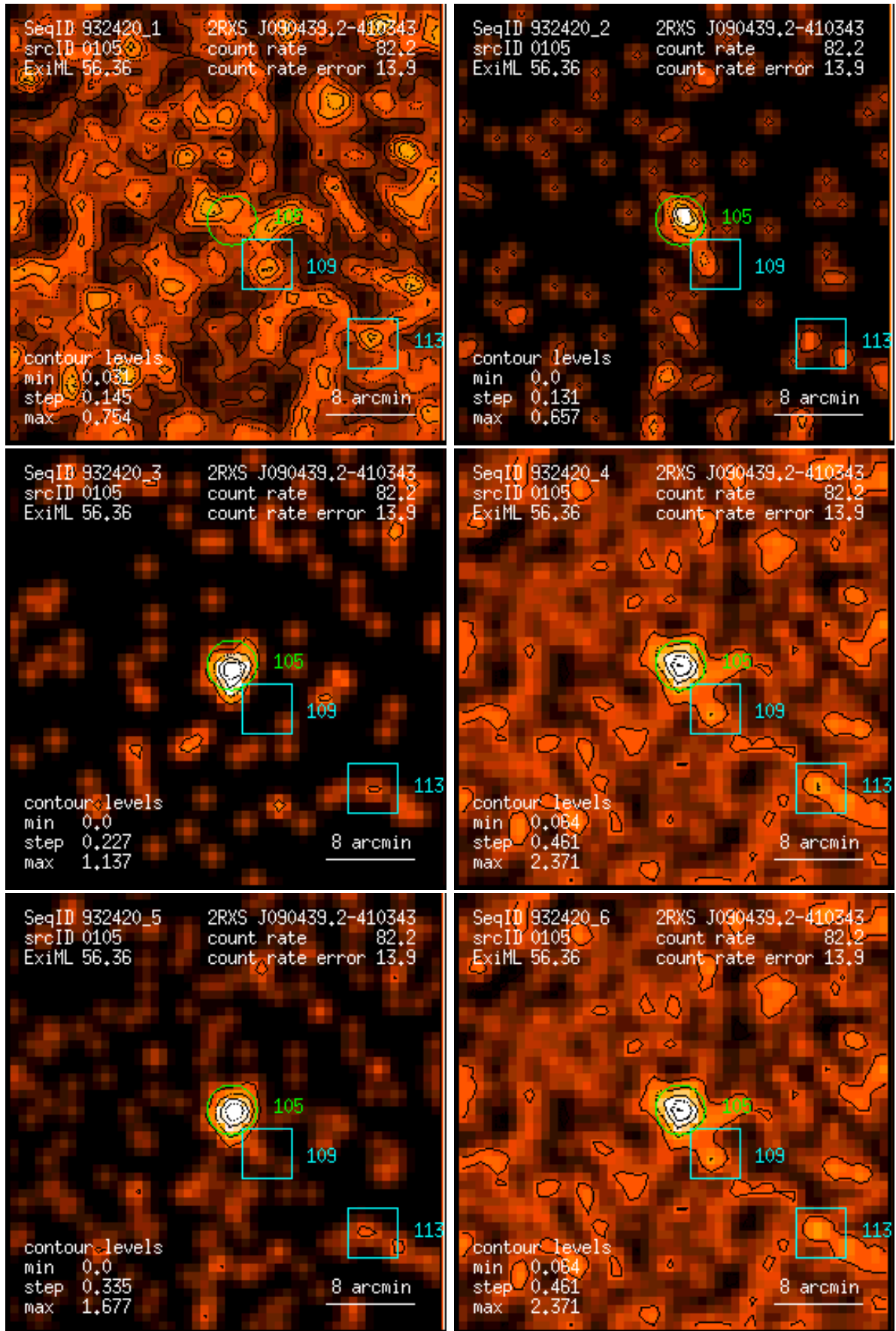
Figure 105: RASS 932420: detection 0105: band rate images, Gaussian filter: (1) PSPC channels 11 – 41, (2) 52 – 90, (3) 91 – 201, (4) 11 – 235, (5) 52 – 201, (6) 11 – 201. Broad band rates in counts/ks. Band rate contour levels in counts/ks/arcmin 2 .
