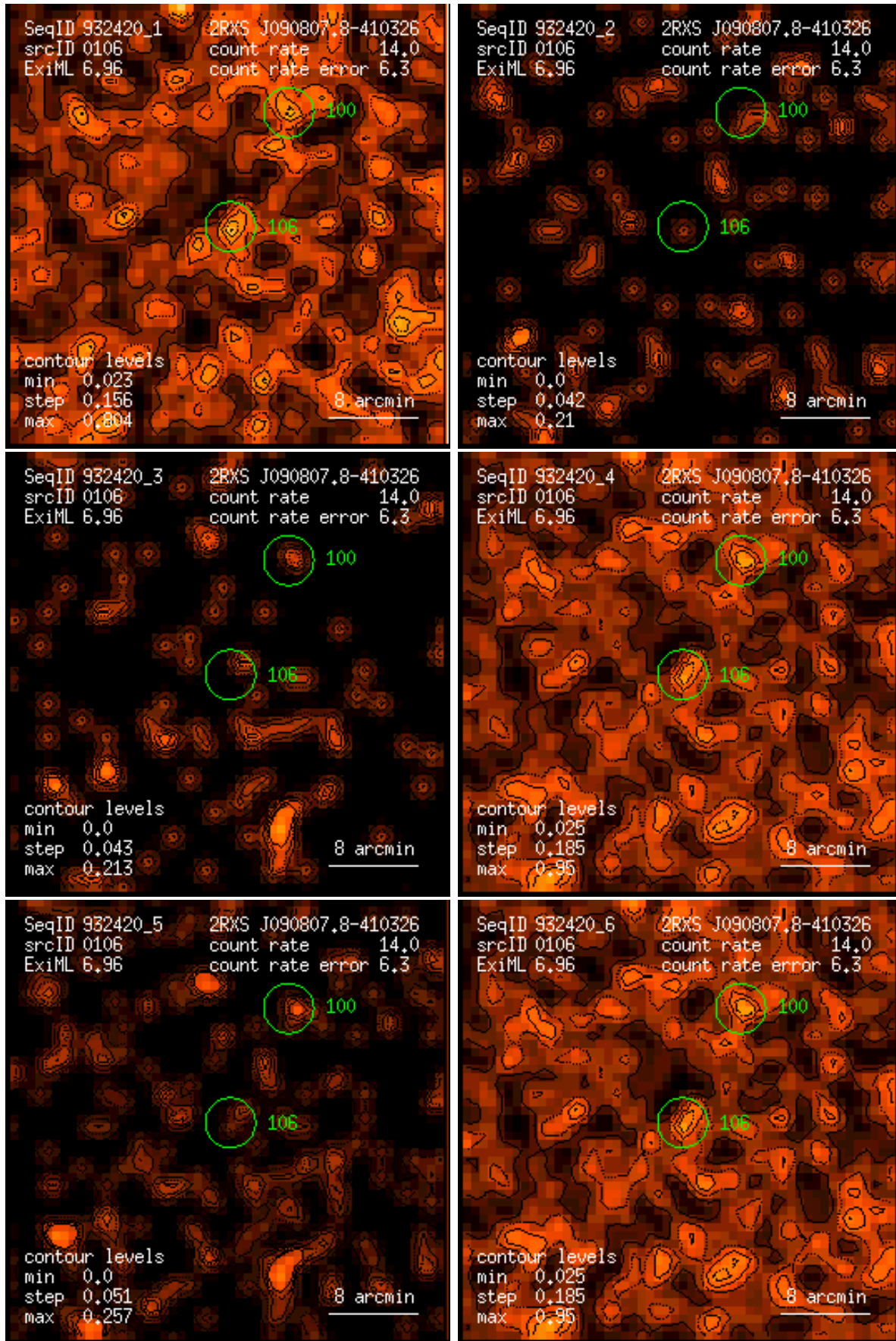
Figure 106: RASS 932420: detection 0106: band rate images, Gaussian filter: (1) PSPC channels 11 – 41, (2) 52 – 90, (3) 91 – 201, (4) 11 – 235, (5) 52 – 201, (6) 11 – 201. Broad band rates in counts/ks. Band rate contour levels in counts/ks/arcmin 2 .
