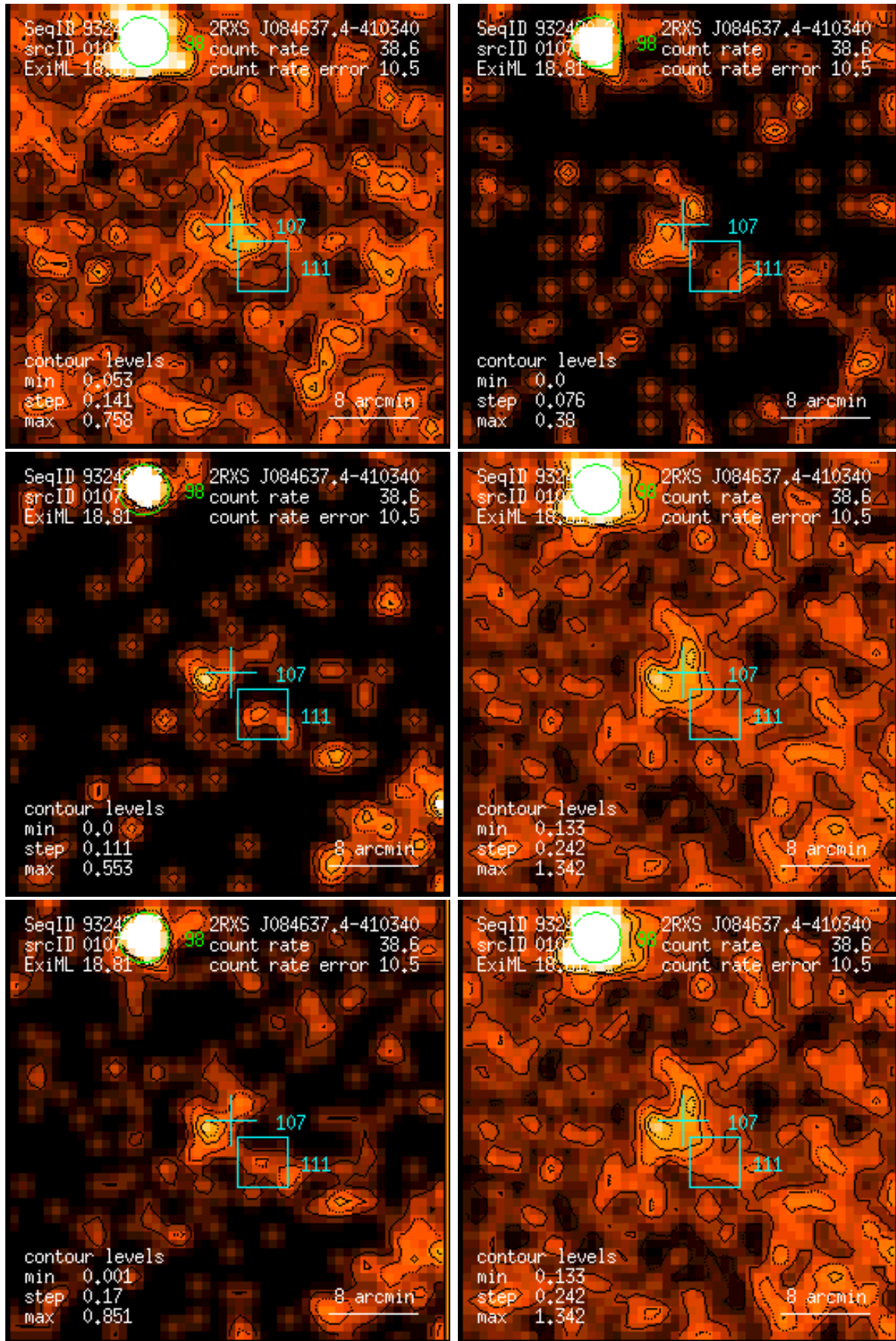
Figure 107: RASS 932420: detection 0107: band rate images, Gaussian filter: (1) PSPC channels 11 – 41, (2) 52 – 90, (3) 91 – 201, (4) 11 – 235, (5) 52 – 201, (6) 11 – 201. Broad band rates in counts/ks. Band rate contour levels in counts/ks/arcmin 2 .
