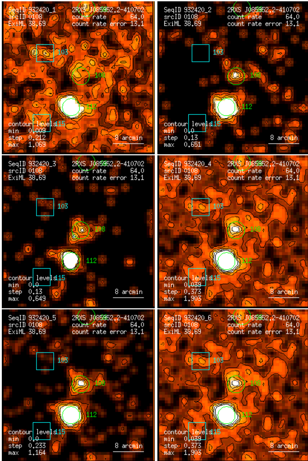
Figure 108: RASS 932420: detection 0108: band rate images, Gaussian filter: (1) PSPC channels 11 – 41, (2) 52 – 90, (3) 91 – 201, (4) 11 – 235, (5) 52 – 201, (6) 11 – 201. Broad band rates in counts/ks. Band rate contour levels in counts/ks/arcmin 2 .
