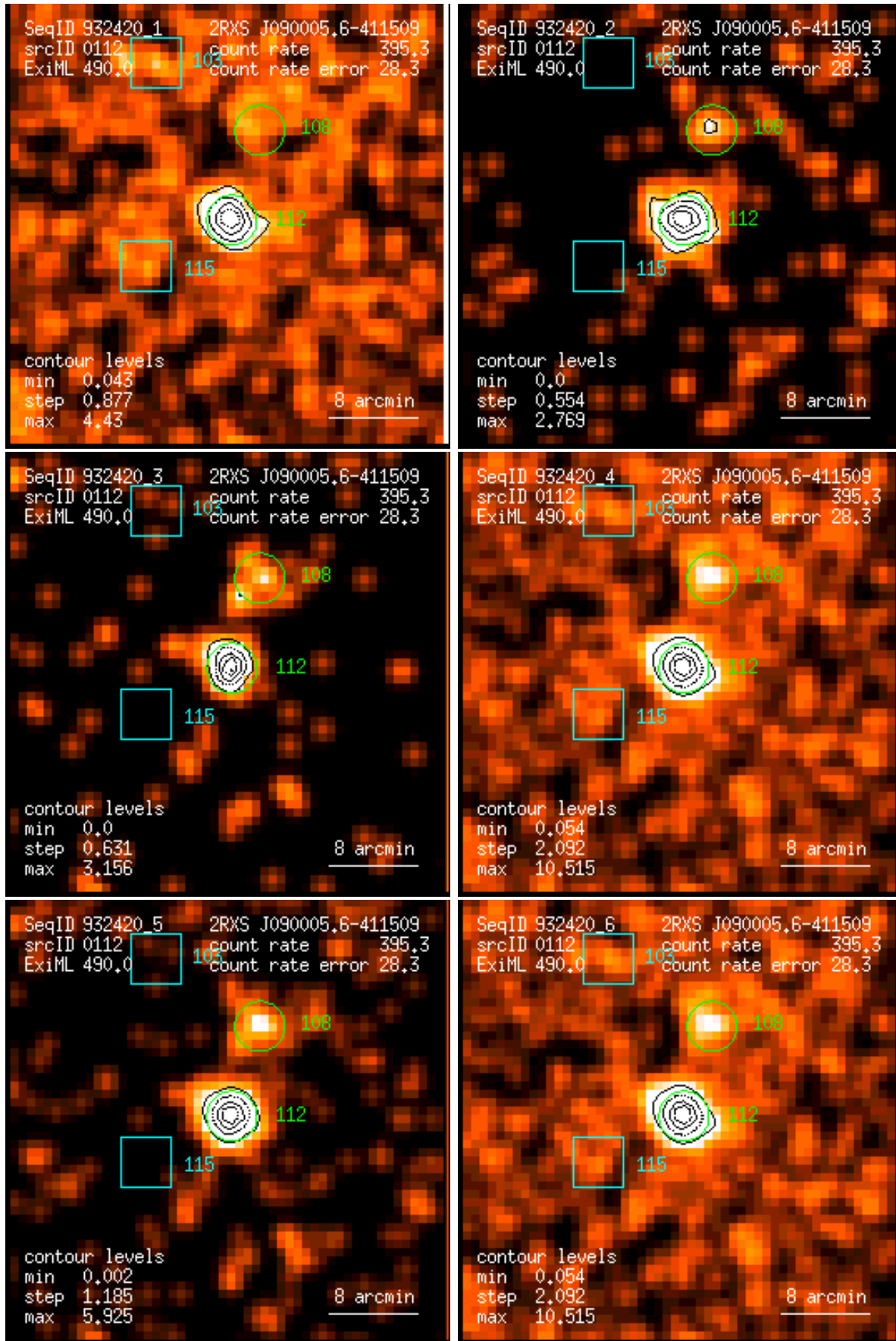
Figure 112: RASS 932420: detection 0112: band rate images, Gaussian filter: (1) PSPC channels 11 – 41, (2) 52 – 90, (3) 91 – 201, (4) 11 – 235, (5) 52 – 201, (6) 11 – 201. Broad band rates in counts/ks. Band rate contour levels in counts/ks/arcmin 2 .
