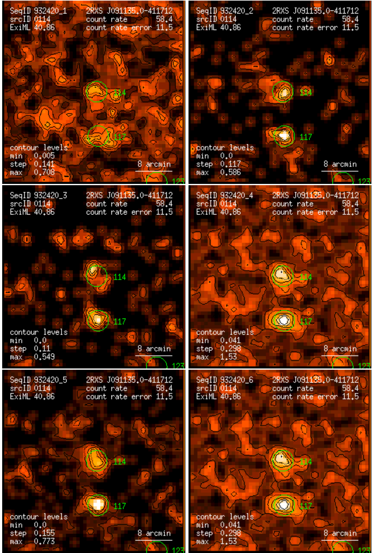
Figure 114: RASS 932420: detection 0114: band rate images, Gaussian filter: (1) PSPC channels 11 – 41, (2) 52 – 90, (3) 91 – 201, (4) 11 – 235, (5) 52 – 201, (6) 11 – 201. Broad band rates in counts/ks. Band rate contour levels in counts/ks/arcmin 2 .
