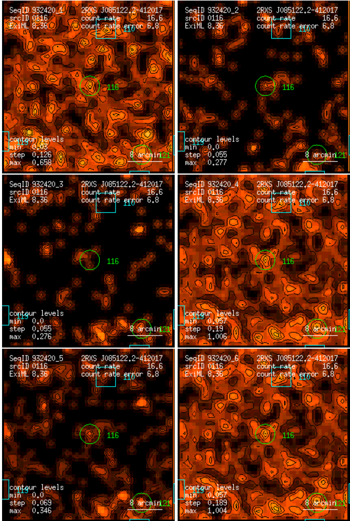
Figure 116: RASS 932420: detection 0116: band rate images, Gaussian filter: (1) PSPC channels 11 – 41, (2) 52 – 90, (3) 91 – 201, (4) 11 – 235, (5) 52 – 201, (6) 11 – 201. Broad band rates in counts/ks. Band rate contour levels in counts/ks/arcmin 2 .
