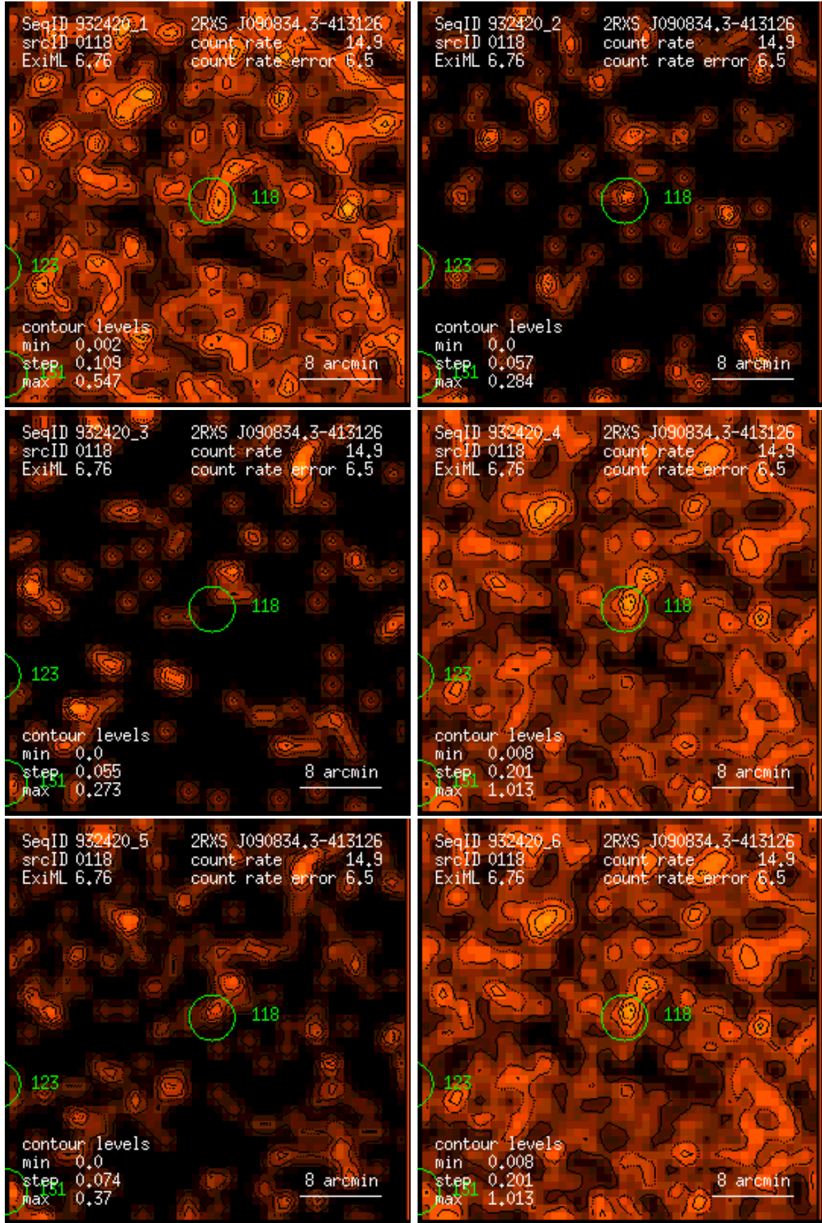
Figure 118: RASS 932420: detection 0118: band rate images, Gaussian filter: (1) PSPC channels 11 – 41, (2) 52 – 90, (3) 91 – 201, (4) 11 – 235, (5) 52 – 201, (6) 11 – 201. Broad band rates in counts/ks. Band rate contour levels in counts/ks/arcmin 2 .
