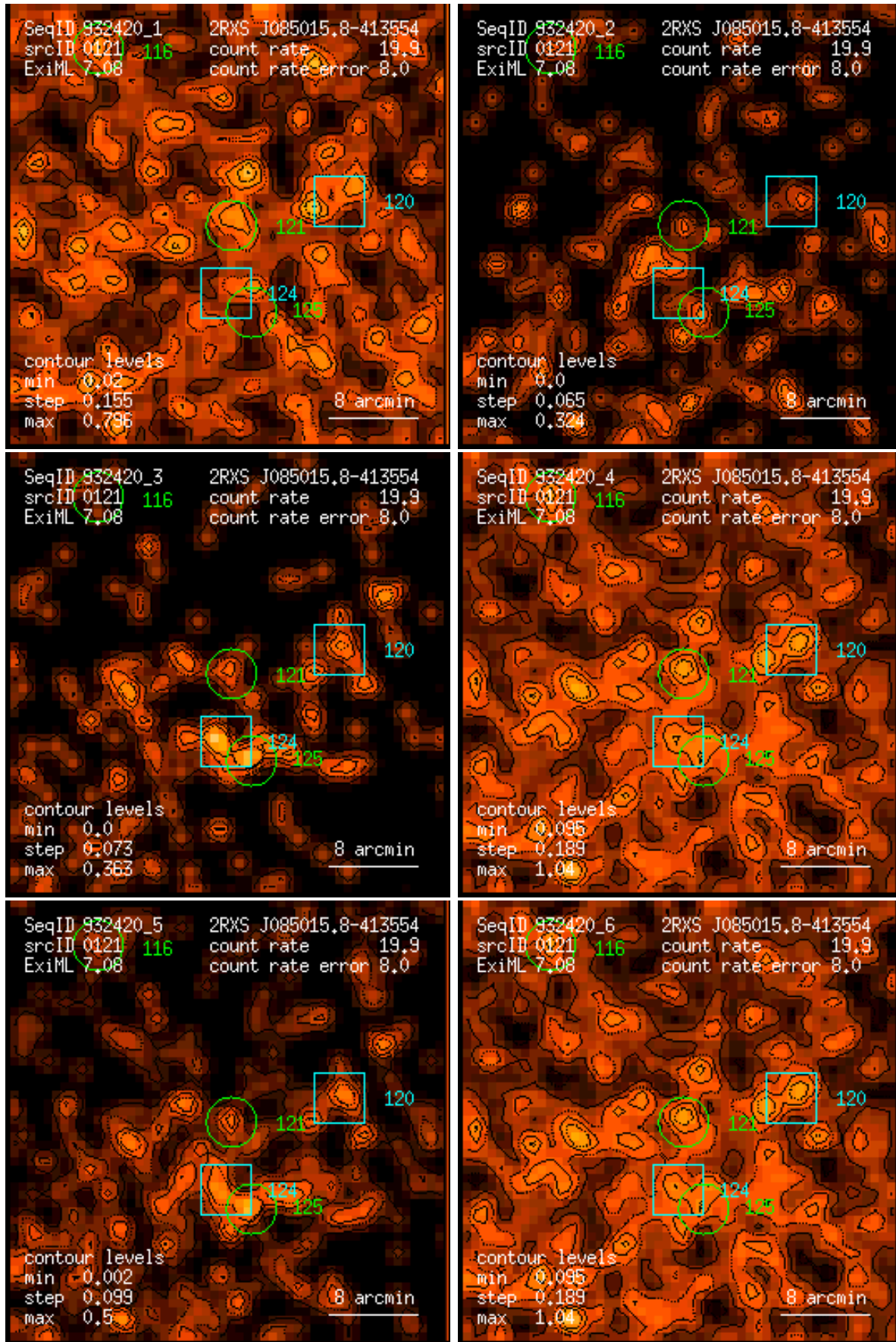
Figure 121: RASS 932420: detection 0121: band rate images, Gaussian filter: (1) PSPC channels 11 – 41, (2) 52 – 90, (3) 91 – 201, (4) 11 – 235, (5) 52 – 201, (6) 11 – 201. Broad band rates in counts/ks. Band rate contour levels in counts/ks/arcmin 2 .
