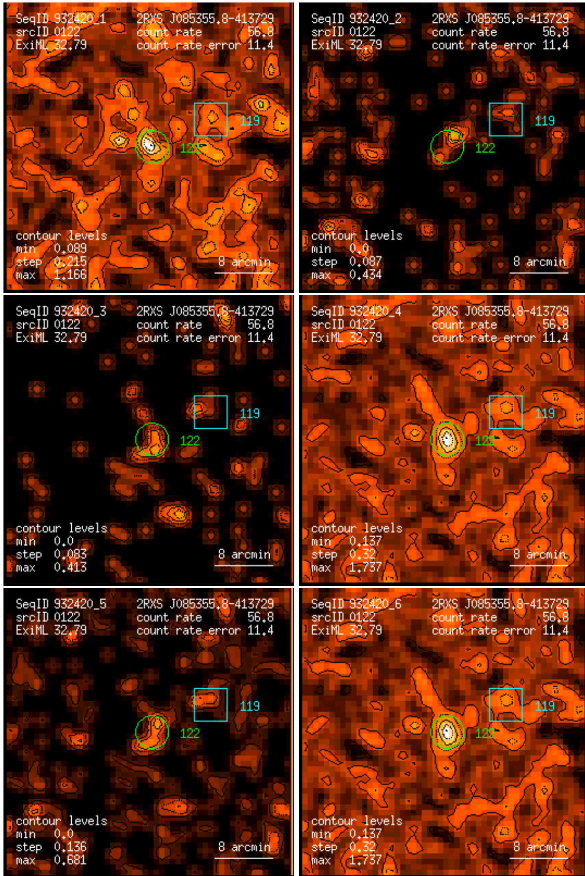
Figure 122: RASS 932420: detection 0122: band rate images, Gaussian filter: (1) PSPC channels 11 – 41, (2) 52 – 90, (3) 91 – 201, (4) 11 – 235, (5) 52 – 201, (6) 11 – 201. Broad band rates in counts/ks. Band rate contour levels in counts/ks/arcmin 2 .
