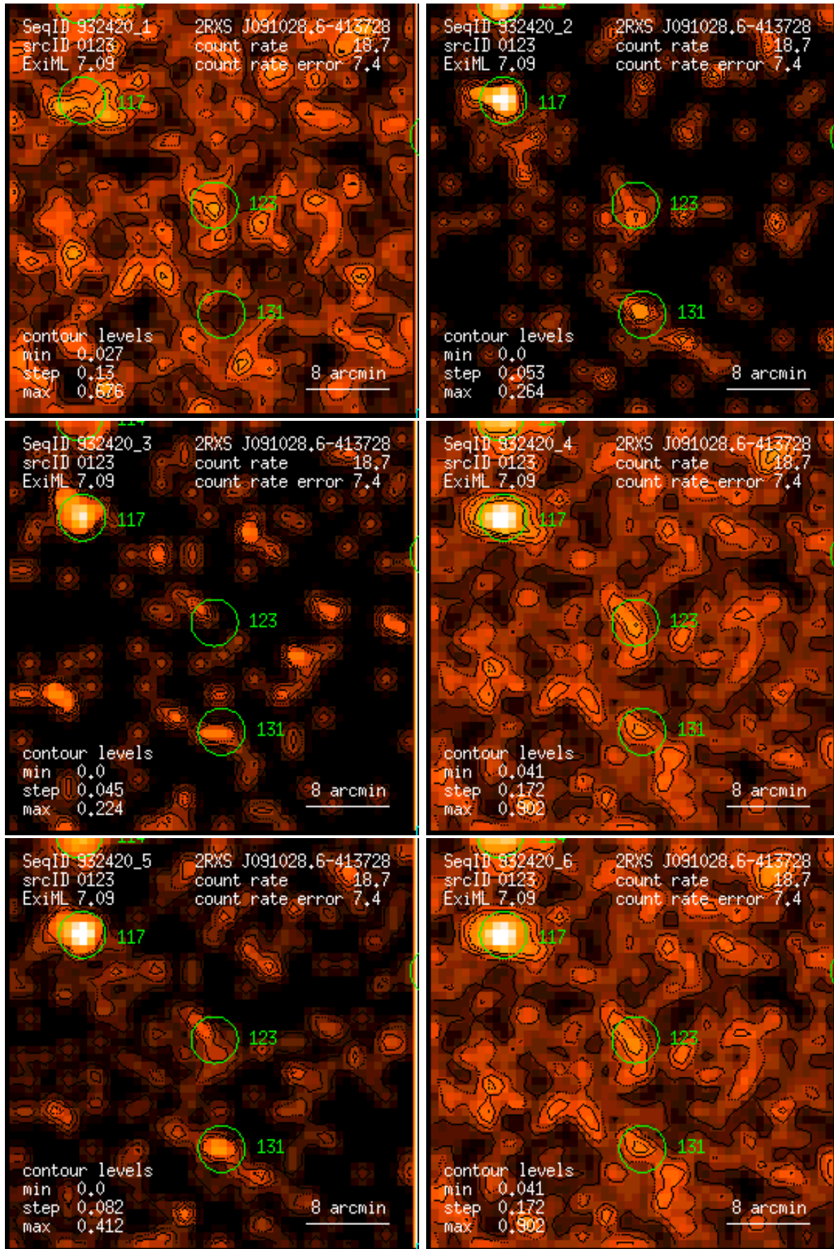
Figure 123: RASS 932420: detection 0123: band rate images, Gaussian filter: (1) PSPC channels 11 – 41, (2) 52 – 90, (3) 91 – 201, (4) 11 – 235, (5) 52 – 201, (6) 11 – 201. Broad band rates in counts/ks. Band rate contour levels in counts/ks/arcmin 2 .
