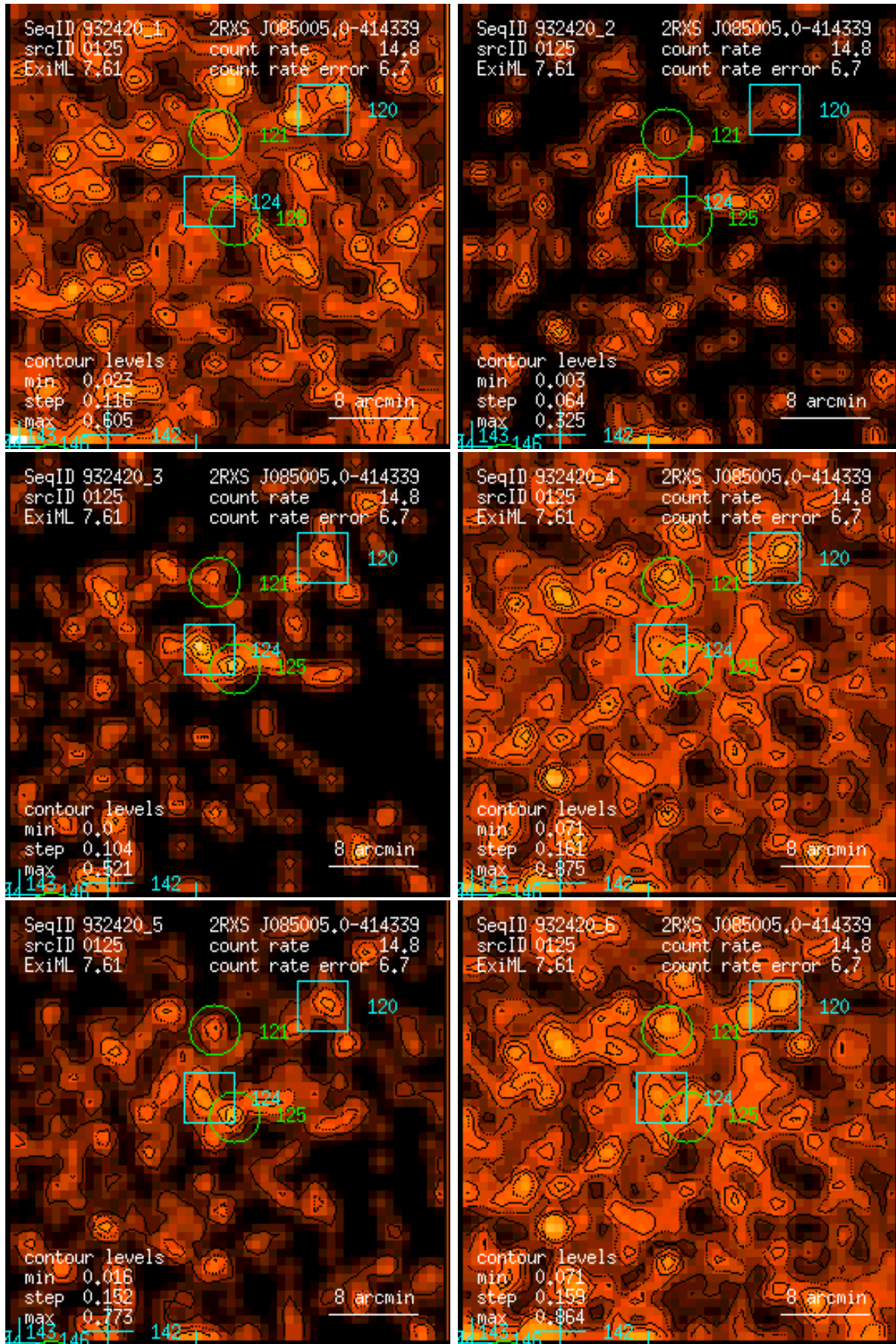
Figure 125: RASS 932420: detection 0125: band rate images, Gaussian filter: (1) PSPC channels 11 – 41, (2) 52 – 90, (3) 91 – 201, (4) 11 – 235, (5) 52 – 201, (6) 11 – 201. Broad band rates in counts/ks. Band rate contour levels in counts/ks/arcmin 2 .
