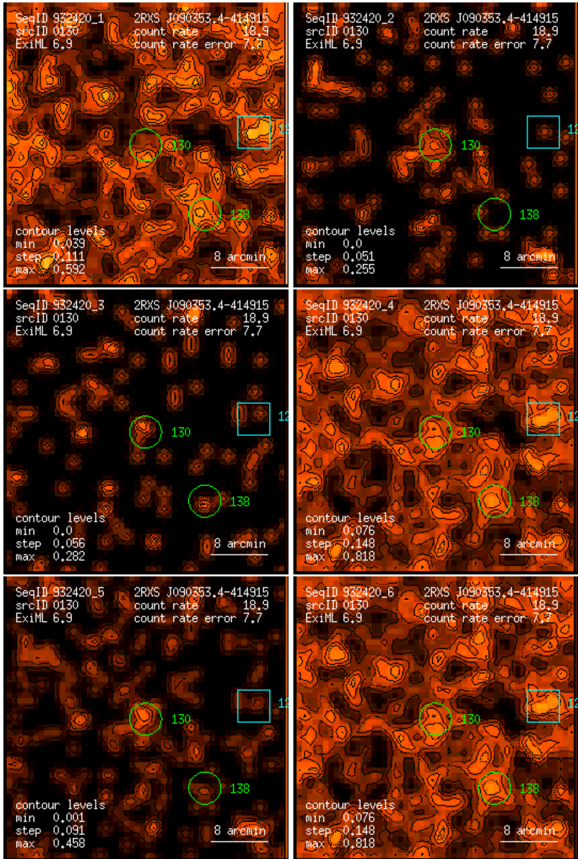
Figure 130: RASS 932420: detection 0130: band rate images, Gaussian filter: (1) PSPC channels 11 – 41, (2) 52 – 90, (3) 91 – 201, (4) 11 – 235, (5) 52 – 201, (6) 11 – 201. Broad band rates in counts/ks. Band rate contour levels in counts/ks/arcmin 2 .
