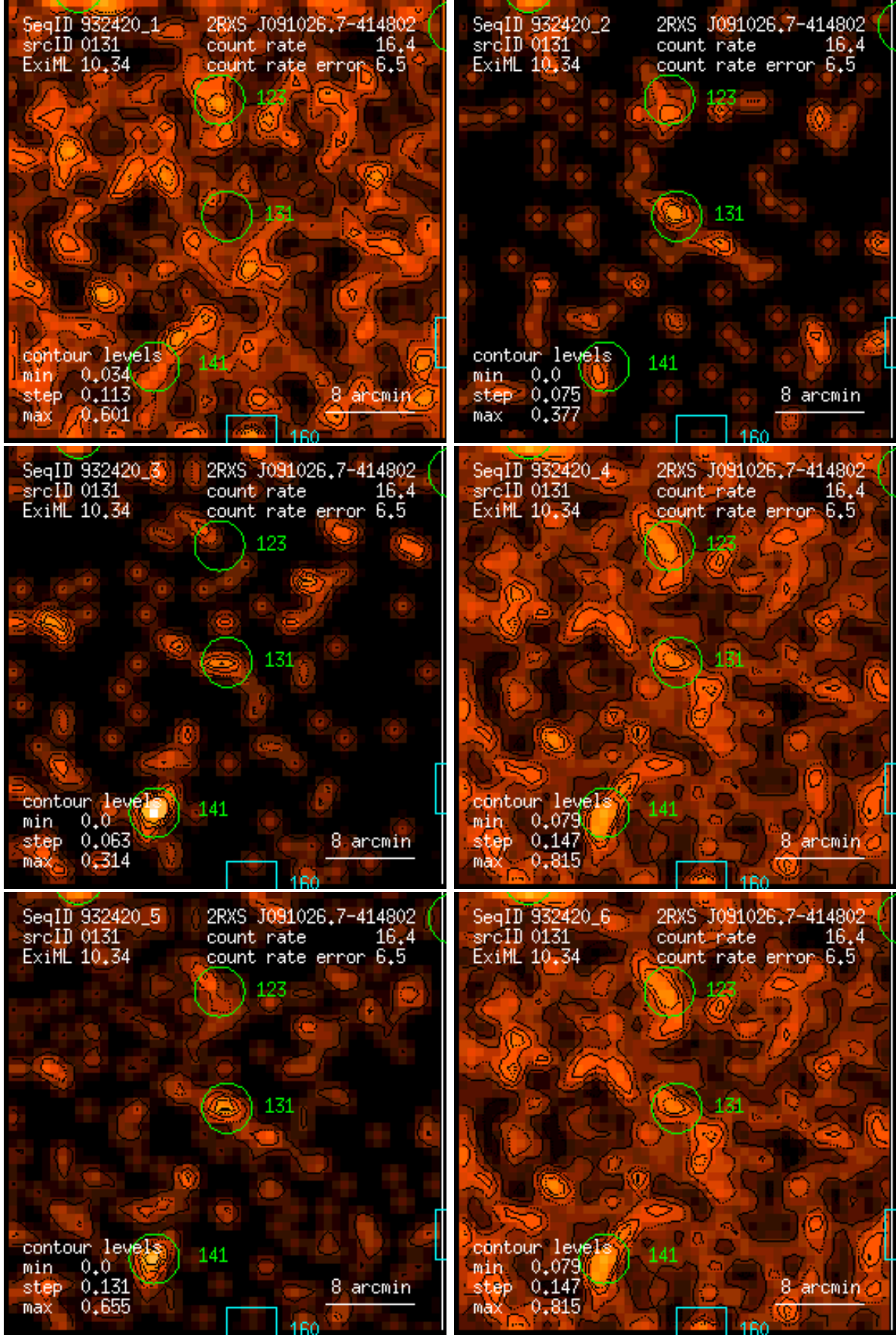
Figure 131: RASS 932420: detection 0131: band rate images, Gaussian filter: (1) PSPC channels 11 – 41, (2) 52 – 90, (3) 91 – 201, (4) 11 – 235, (5) 52 – 201, (6) 11 – 201. Broad band rates in counts/ks. Band rate contour levels in counts/ks/arcmin 2 .
