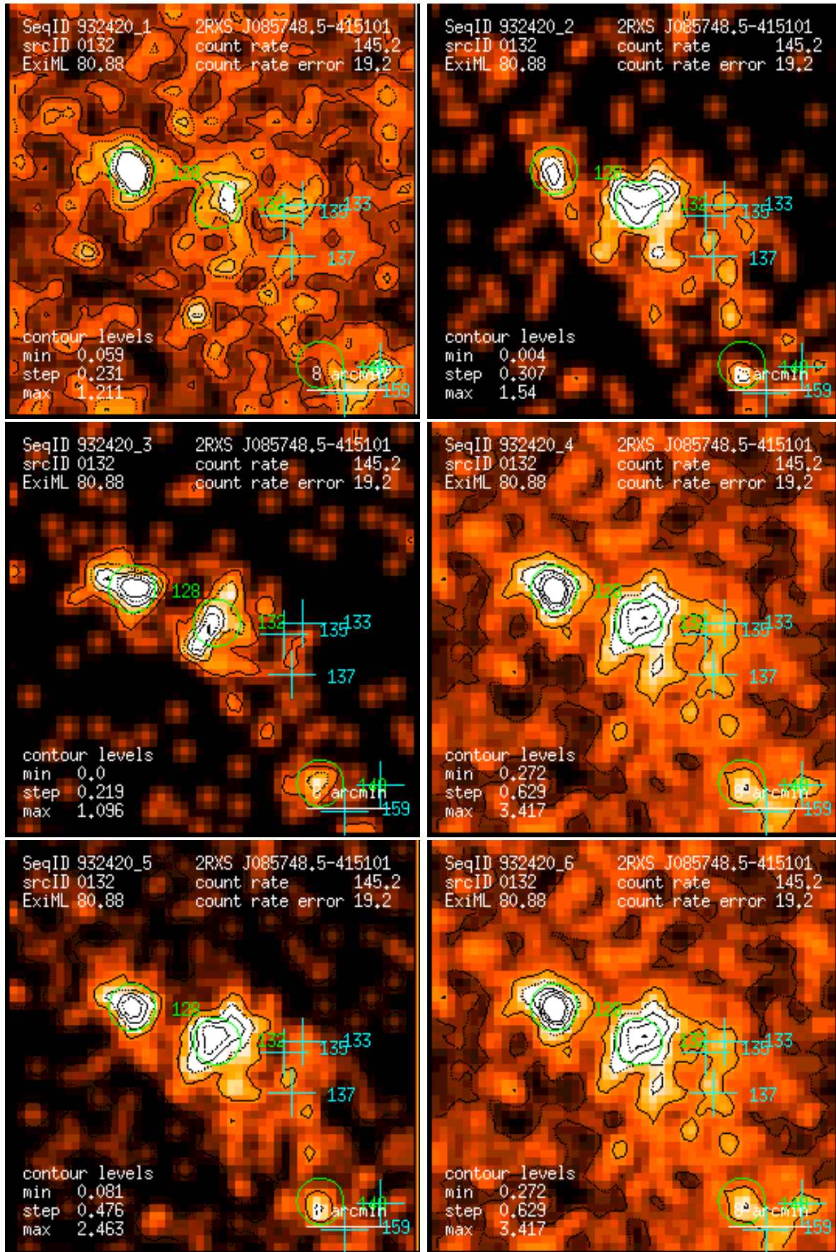
Figure 132: RASS 932420: detection 0132: band rate images, Gaussian filter: (1) PSPC channels 11 – 41, (2) 52 – 90, (3) 91 – 201, (4) 11 – 235, (5) 52 – 201, (6) 11 – 201. Broad band rates in counts/ks. Band rate contour levels in counts/ks/arcmin 2 .
