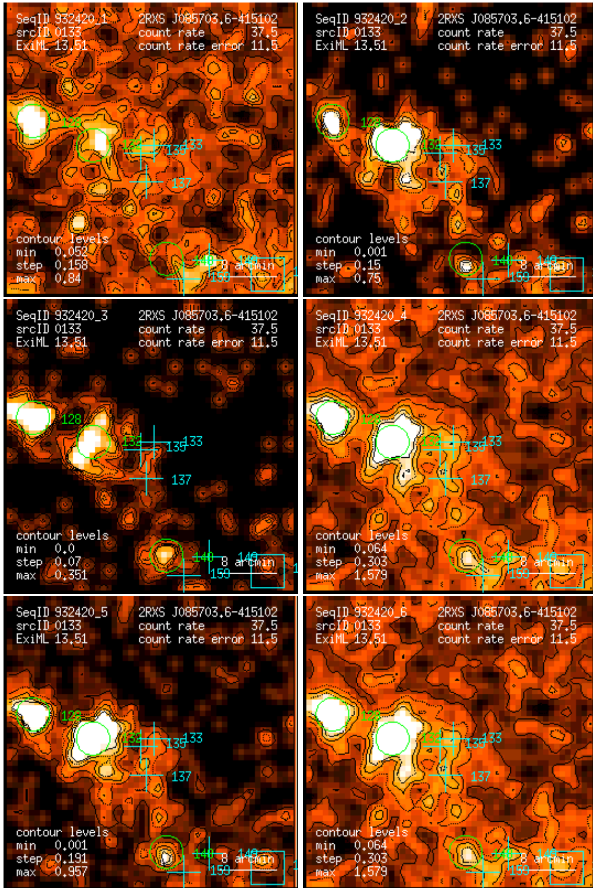
Figure 133: RASS 932420: detection 0133: band rate images, Gaussian filter: (1) PSPC channels 11 – 41, (2) 52 – 90, (3) 91 – 201, (4) 11 – 235, (5) 52 – 201, (6) 11 – 201. Broad band rates in counts/ks. Band rate contour levels in counts/ks/arcmin 2 .
