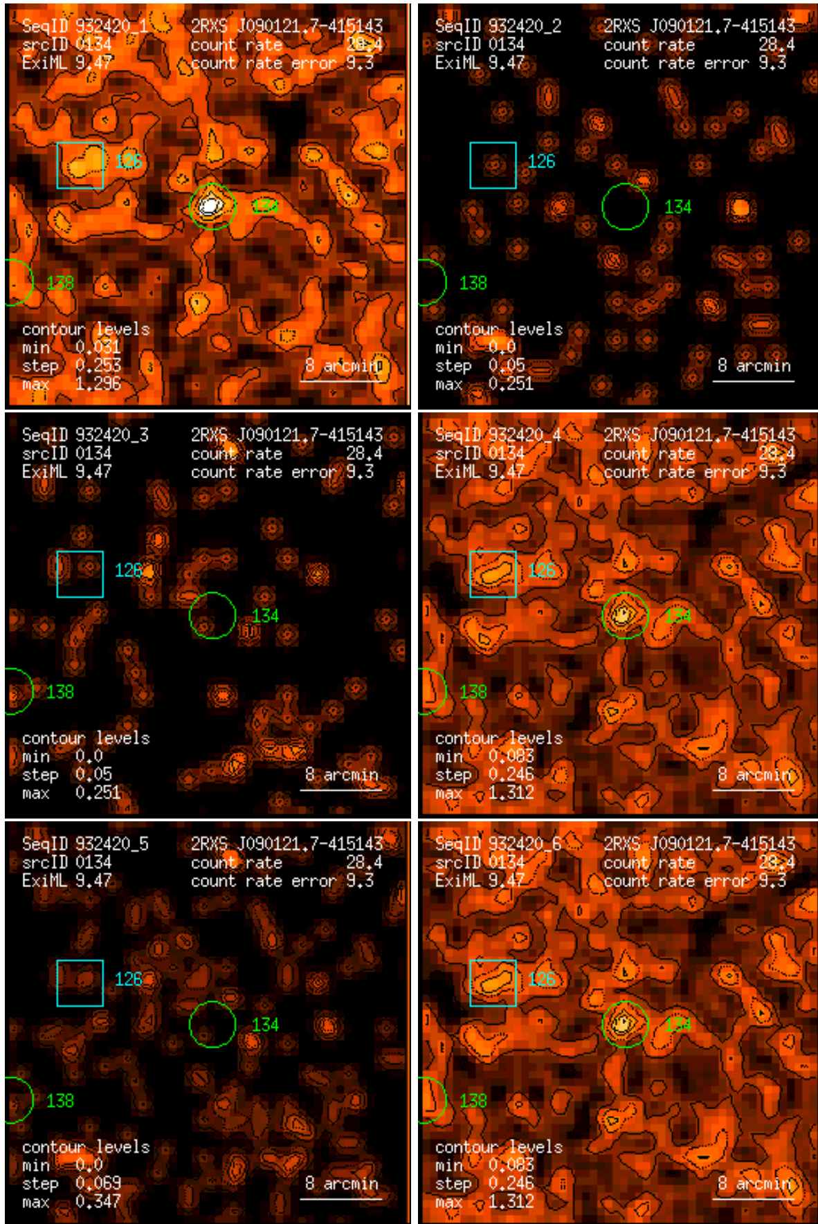
Figure 134: RASS 932420: detection 0134: band rate images, Gaussian filter: (1) PSPC channels 11 – 41, (2) 52 – 90, (3) 91 – 201, (4) 11 – 235, (5) 52 – 201, (6) 11 – 201. Broad band rates in counts/ks. Band rate contour levels in counts/ks/arcmin 2 .
