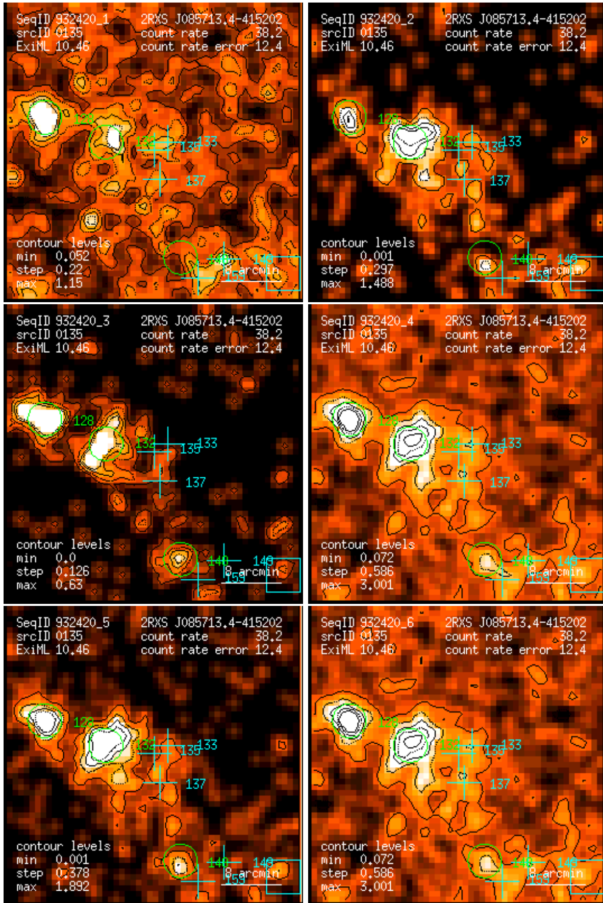
Figure 135: RASS 932420: detection 0135: band rate images, Gaussian filter: (1) PSPC channels 11 – 41, (2) 52 – 90, (3) 91 – 201, (4) 11 – 235, (5) 52 – 201, (6) 11 – 201. Broad band rates in counts/ks. Band rate contour levels in counts/ks/arcmin 2 .
