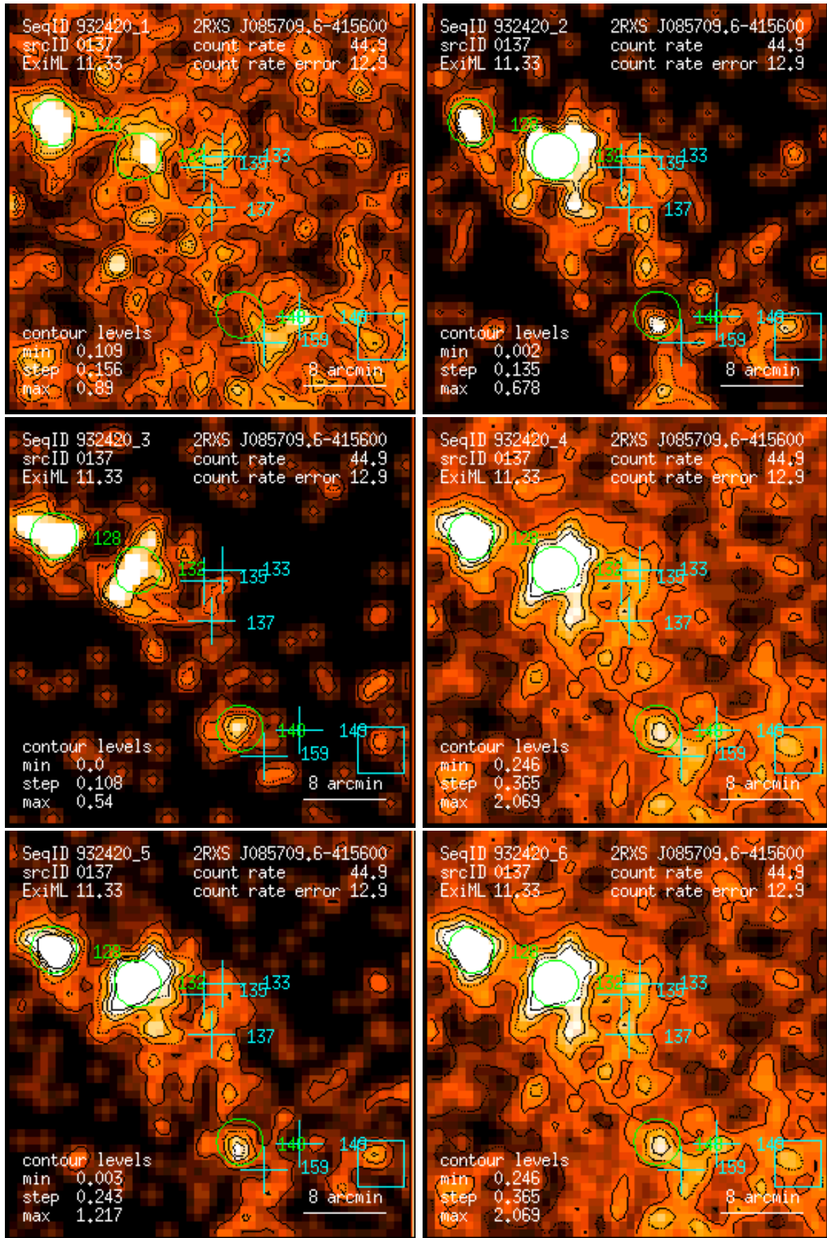
Figure 137: RASS 932420: detection 0137: band rate images, Gaussian filter: (1) PSPC channels 11 – 41, (2) 52 – 90, (3) 91 – 201, (4) 11 – 235, (5) 52 – 201, (6) 11 – 201. Broad band rates in counts/ks. Band rate contour levels in counts/ks/arcmin 2 .
