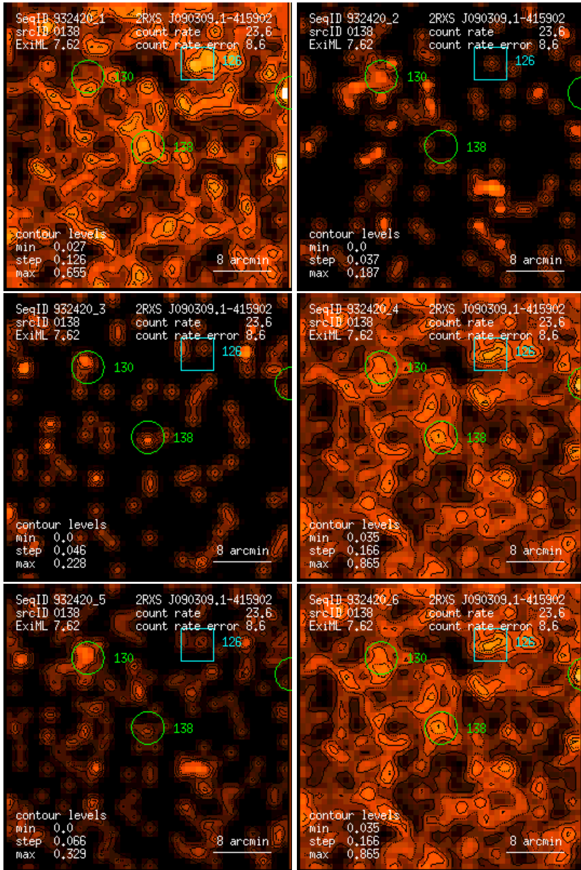
Figure 138: RASS 932420: detection 0138: band rate images, Gaussian filter: (1) PSPC channels 11 – 41, (2) 52 – 90, (3) 91 – 201, (4) 11 – 235, (5) 52 – 201, (6) 11 – 201. Broad band rates in counts/ks. Band rate contour levels in counts/ks/arcmin 2 .
