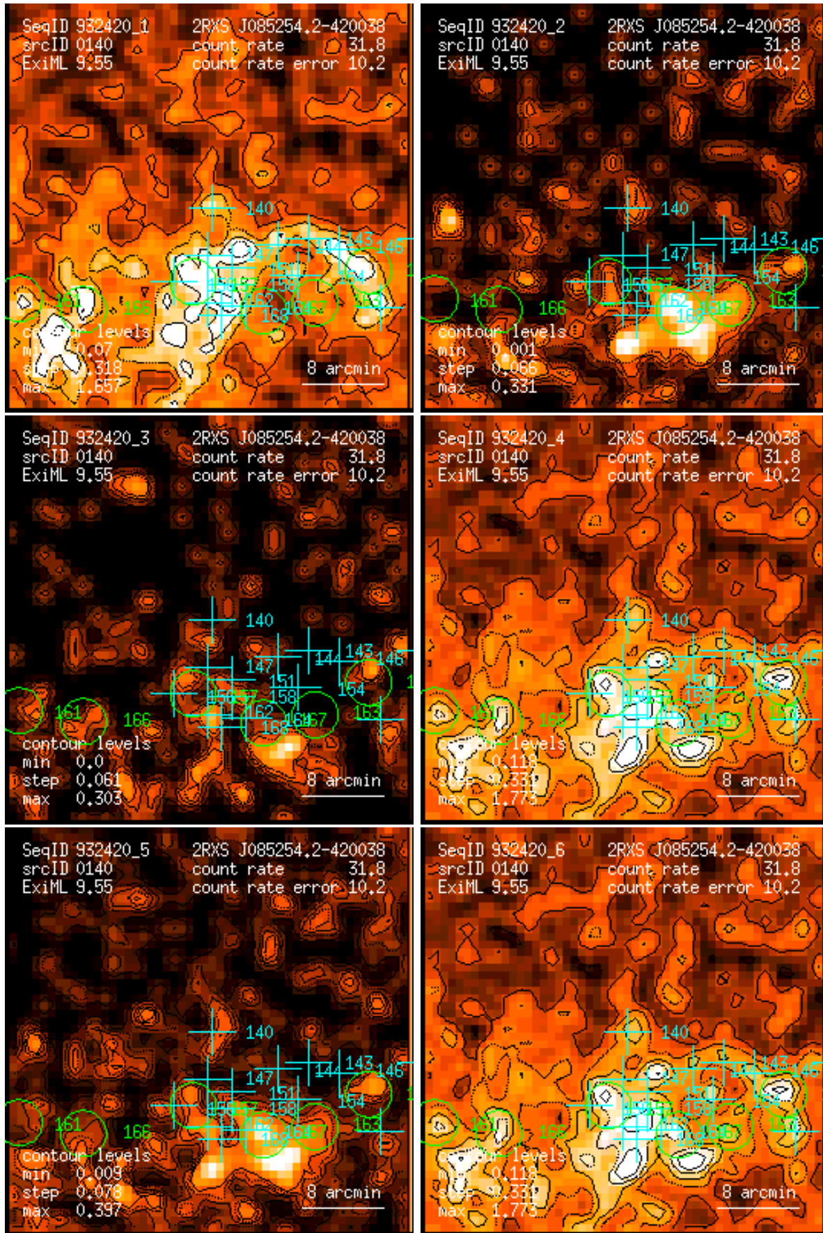
Figure 140: RASS 932420: detection 0140: band rate images, Gaussian filter: (1) PSPC channels 11 – 41, (2) 52 – 90, (3) 91 – 201, (4) 11 – 235, (5) 52 – 201, (6) 11 – 201. Broad band rates in counts/ks. Band rate contour levels in counts/ks/arcmin 2 .
