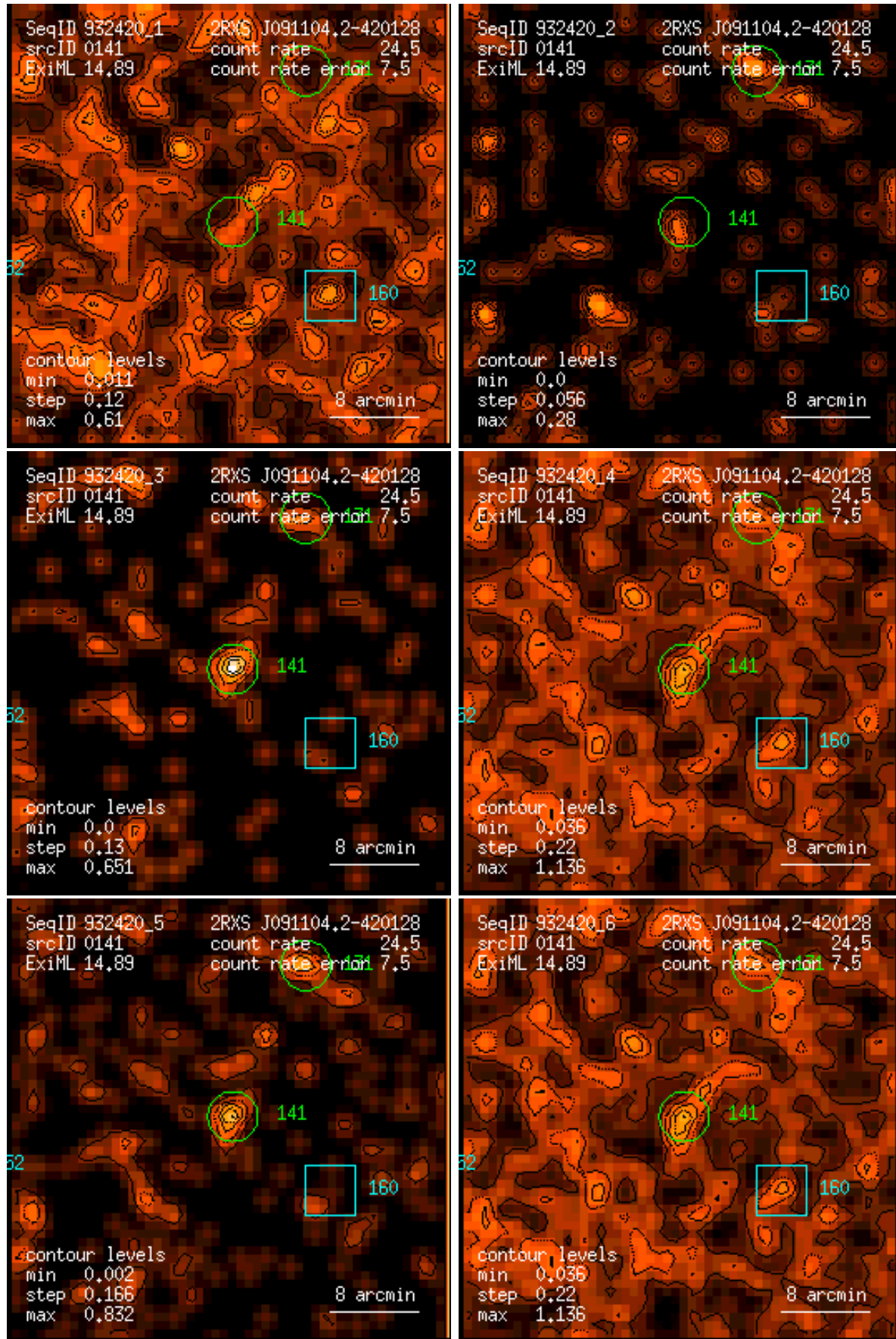
Figure 141: RASS 932420: detection 0141: band rate images, Gaussian filter: (1) PSPC channels 11 – 41, (2) 52 – 90, (3) 91 – 201, (4) 11 – 235, (5) 52 – 201, (6) 11 – 201. Broad band rates in counts/ks. Band rate contour levels in counts/ks/arcmin 2 .
