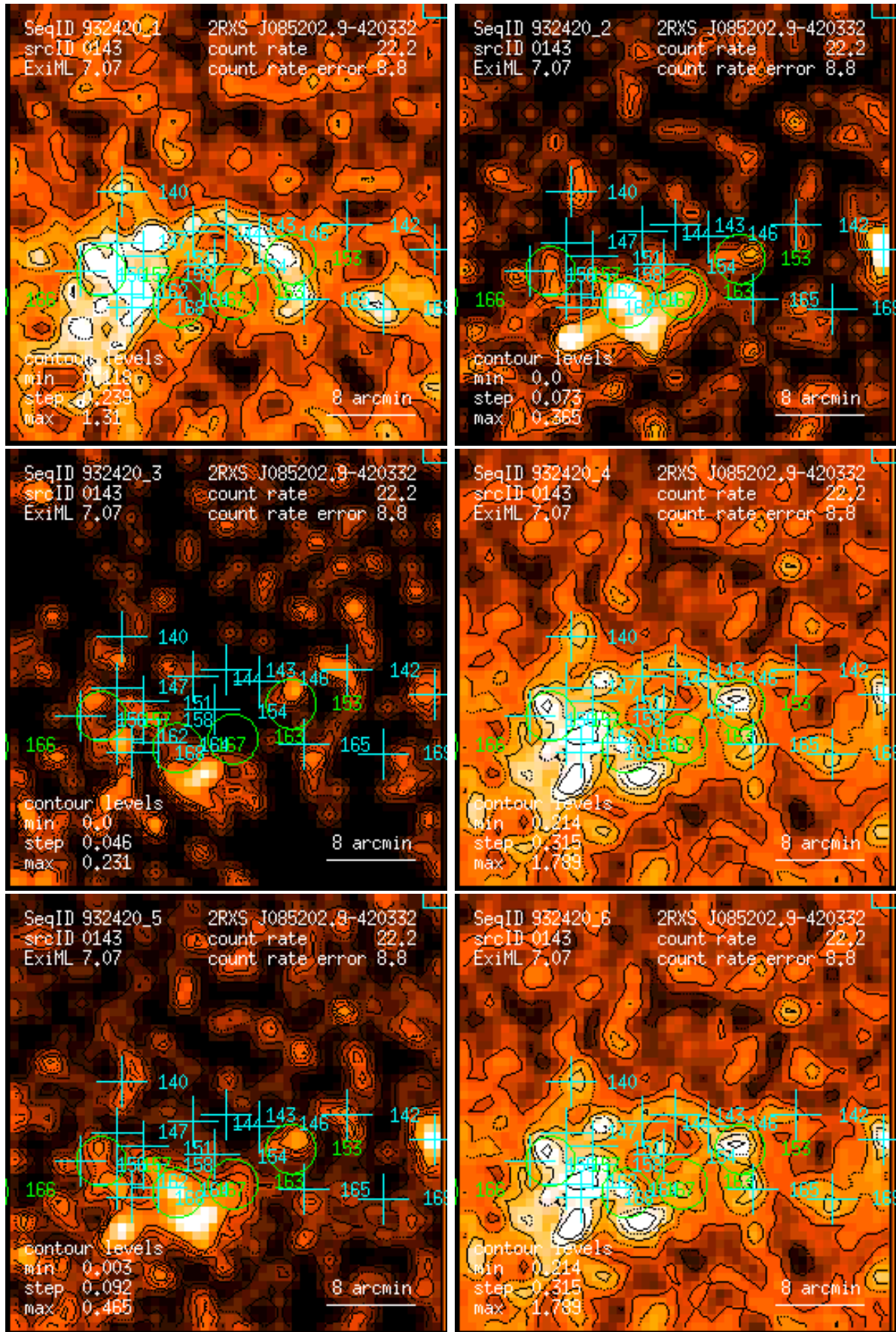
Figure 143: RASS 932420: detection 0143: band rate images, Gaussian filter: (1) PSPC channels 11 – 41, (2) 52 – 90, (3) 91 – 201, (4) 11 – 235, (5) 52 – 201, (6) 11 – 201. Broad band rates in counts/ks. Band rate contour levels in counts/ks/arcmin 2 .
